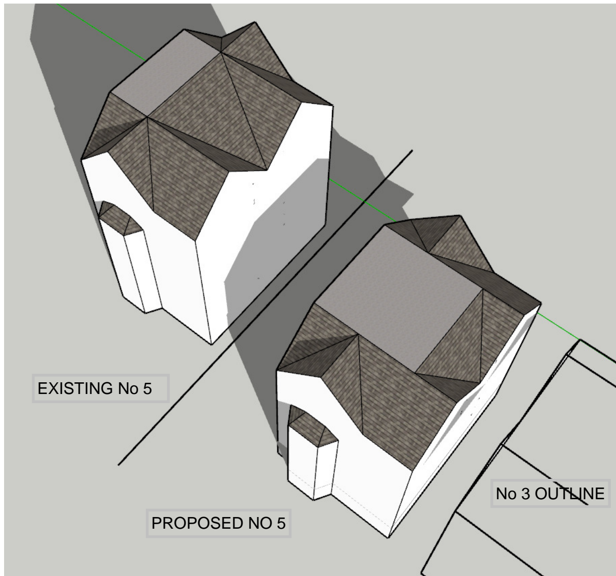
BIRDS EYE VIEW OF ROOF FROM FRONT EXISTING ON LHS PROPOSED ON RHS No 3 IN OUTLINE
