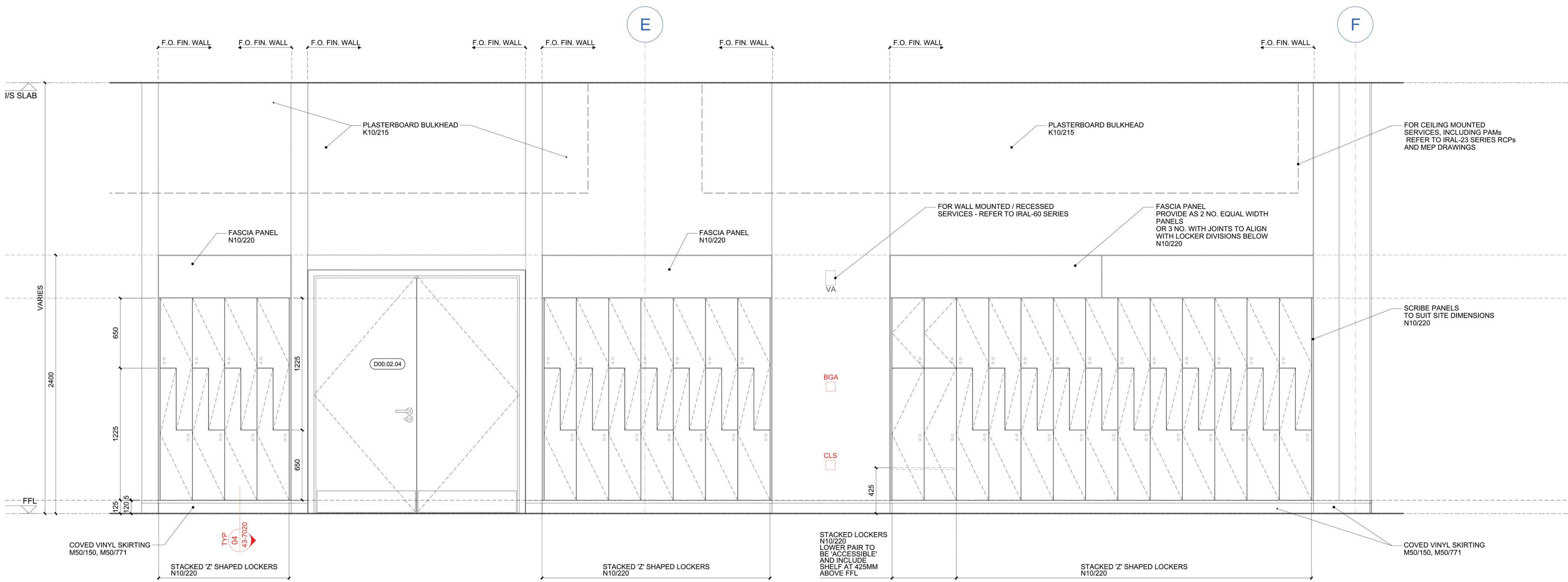
Ground Floor Locker Elevation 1:20
