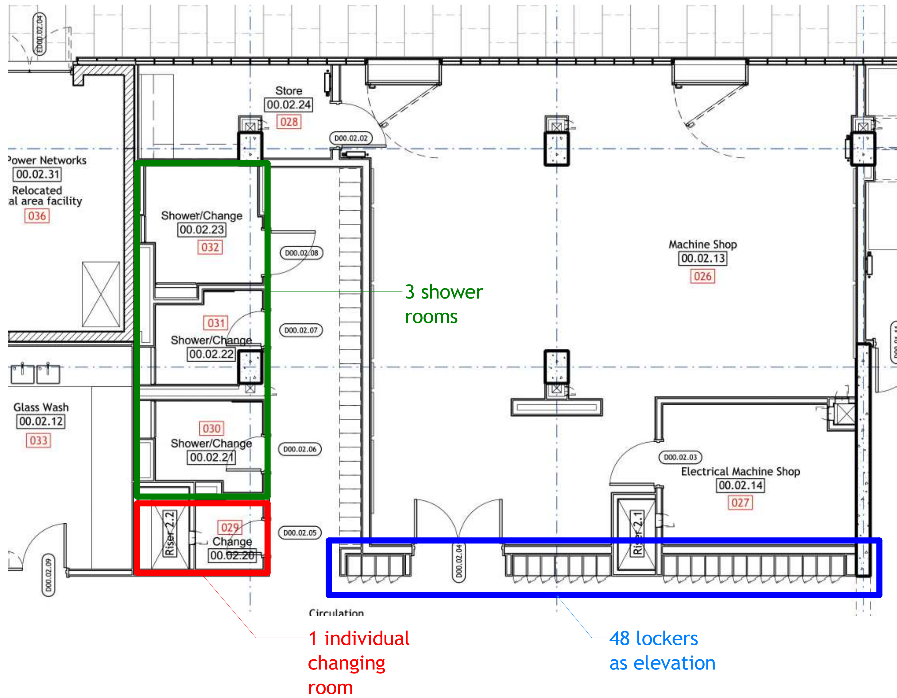
Ground Floor Changing Rooms & Showers 1:50
