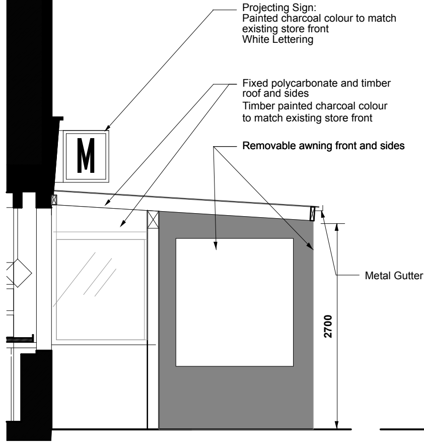
B PROPOSED SIDE ELEVATION S205 1:50
