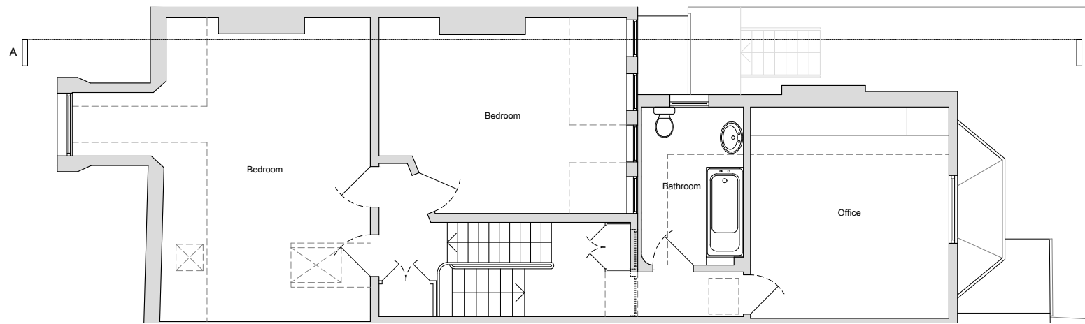
SECOND FLOOR
