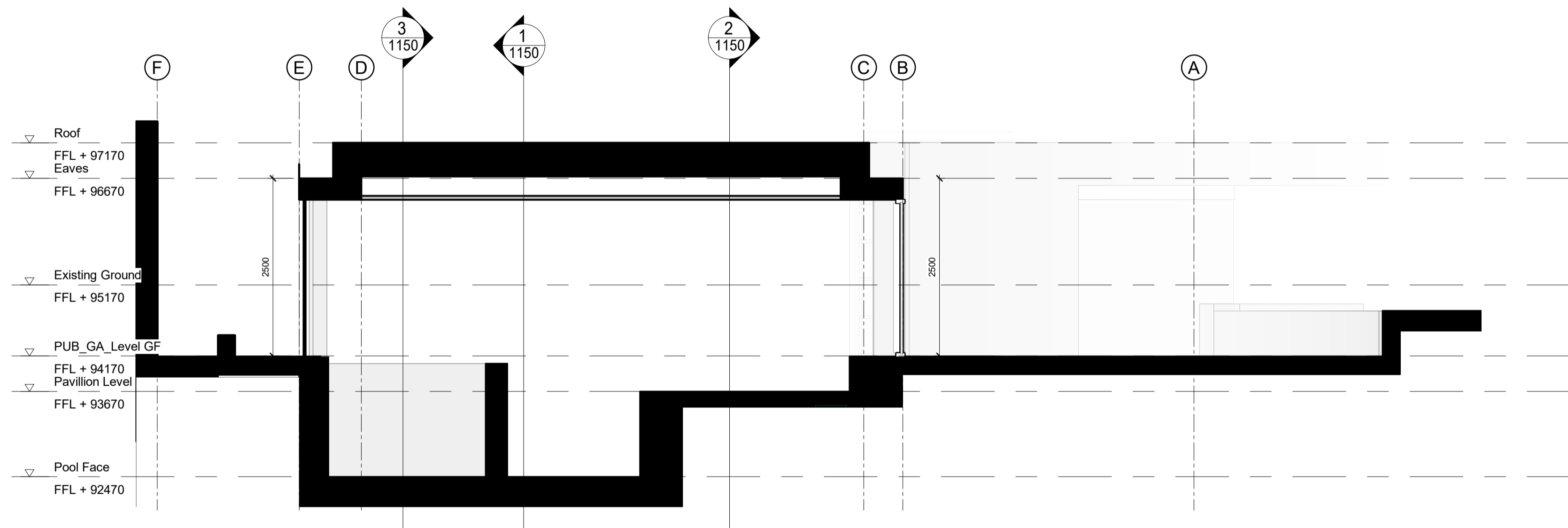
Proposed Section B2 1 : 50
