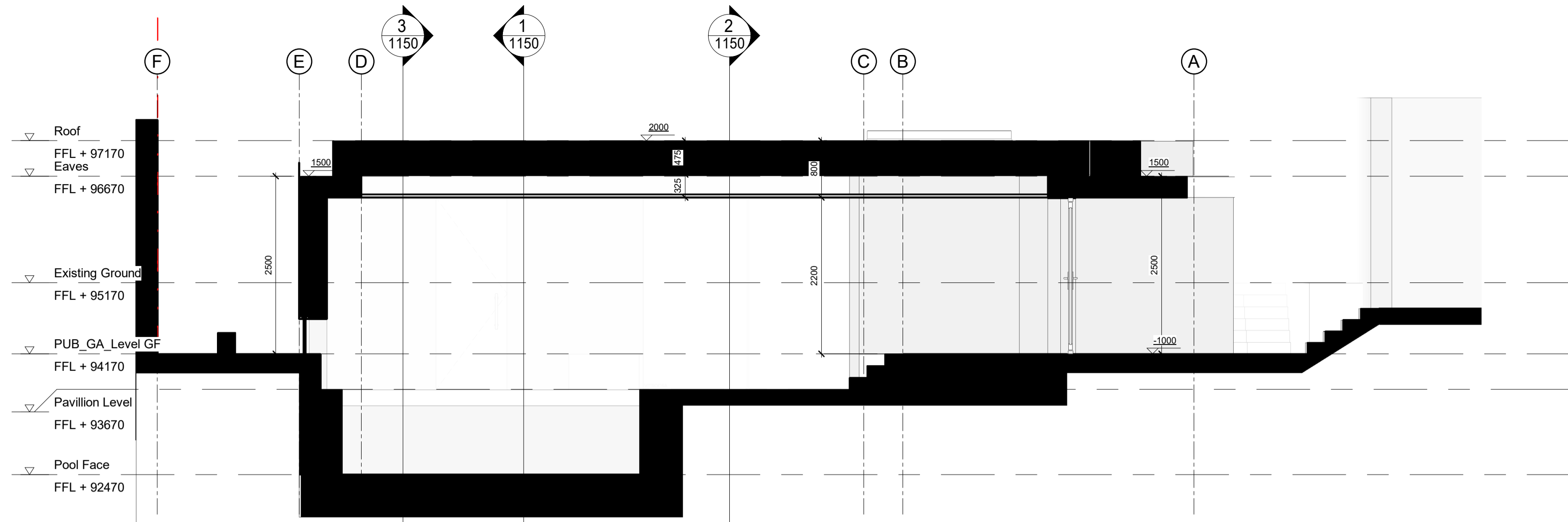
Proposed Section B1 1 : 50
