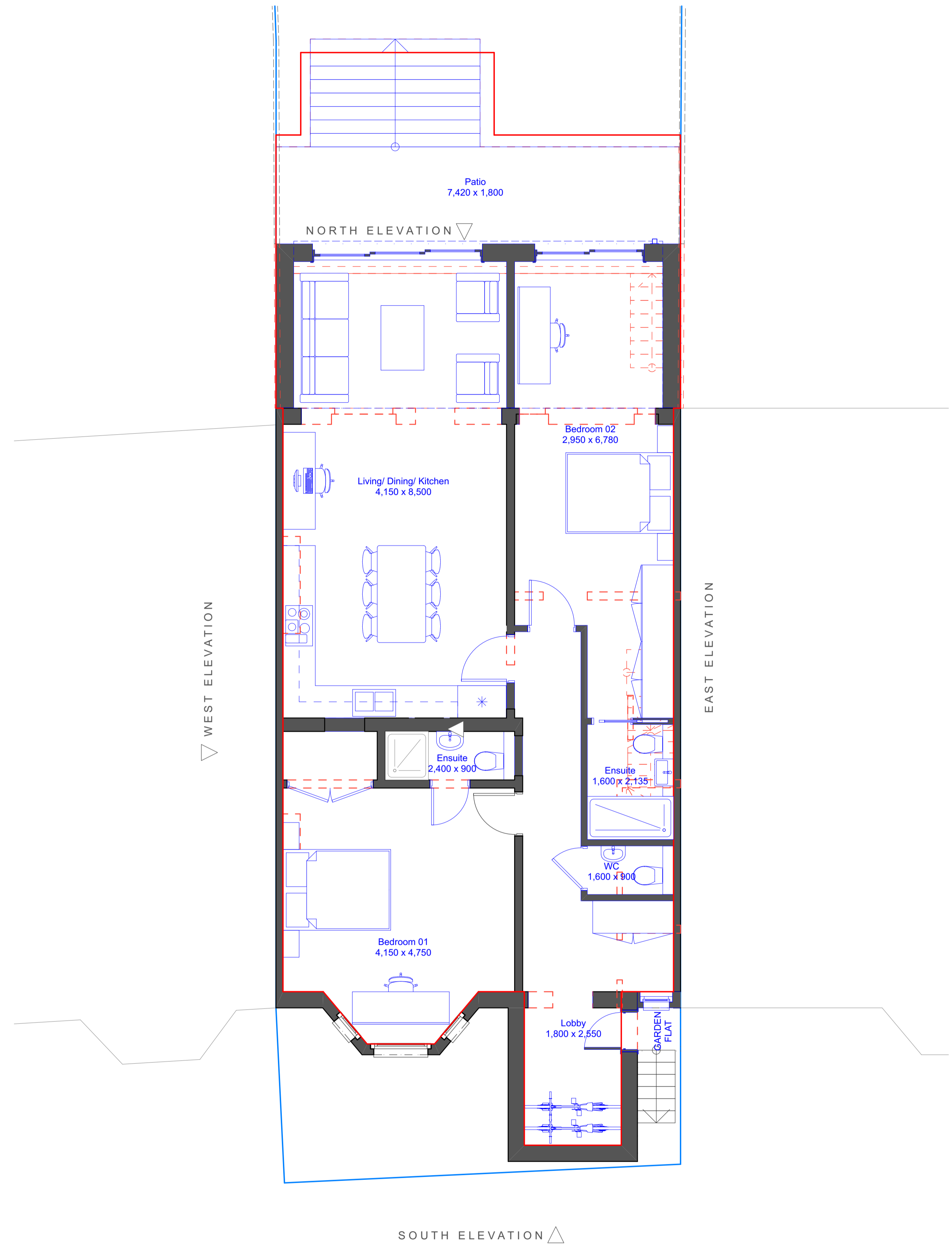
PROPOSED LOWER 1:50
