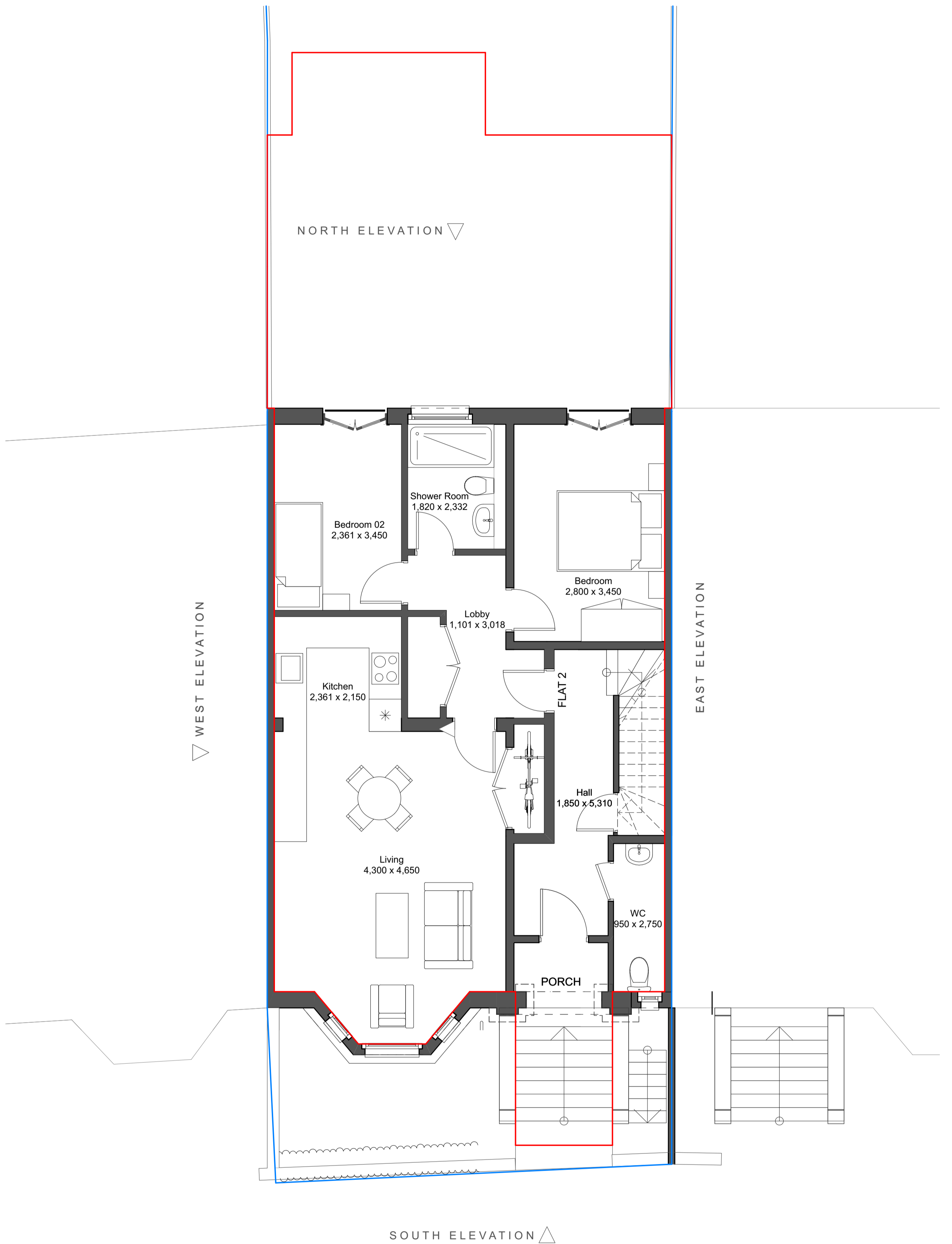
EXISTING GROUND 1:50
