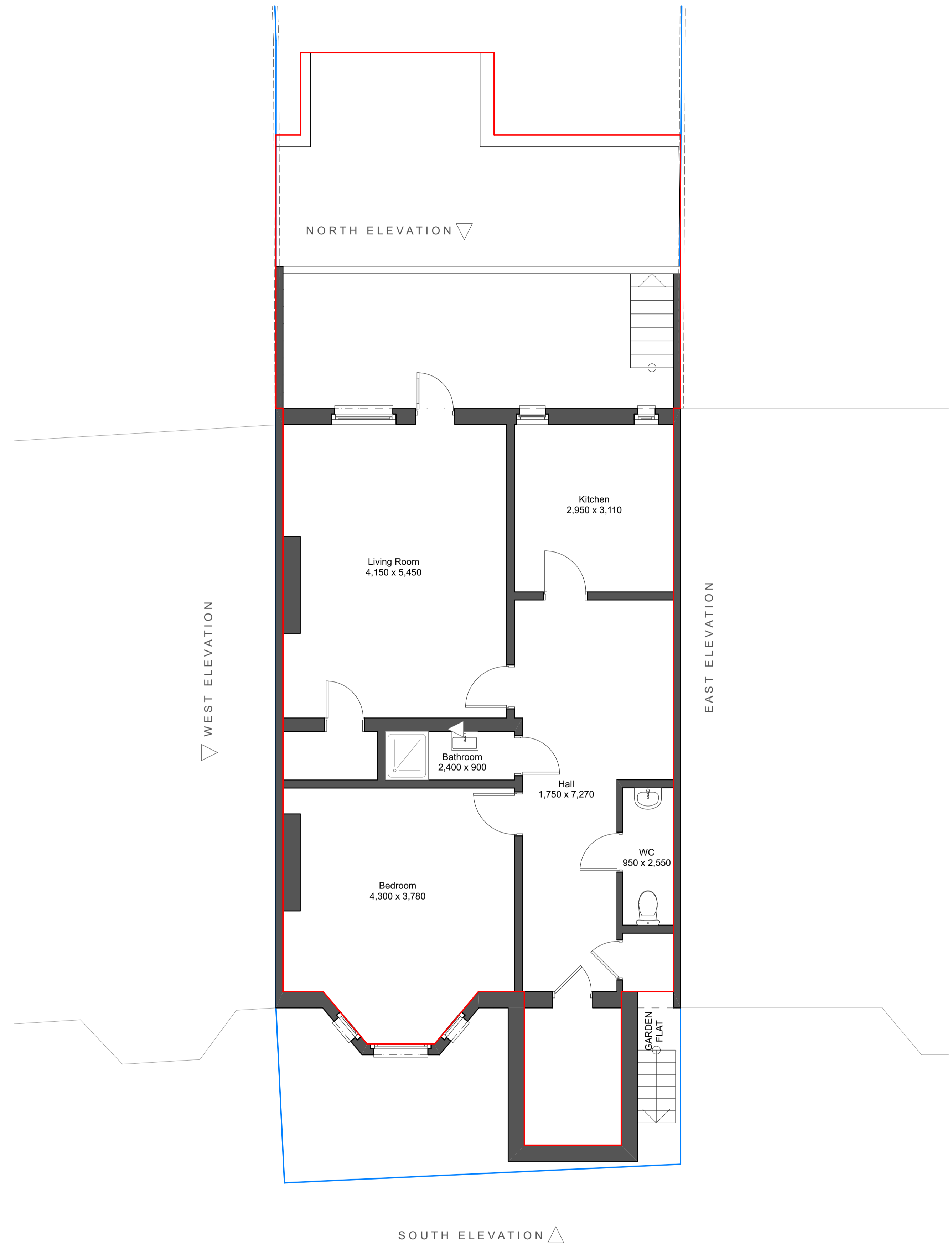
EXISTING LOWER 1:50
