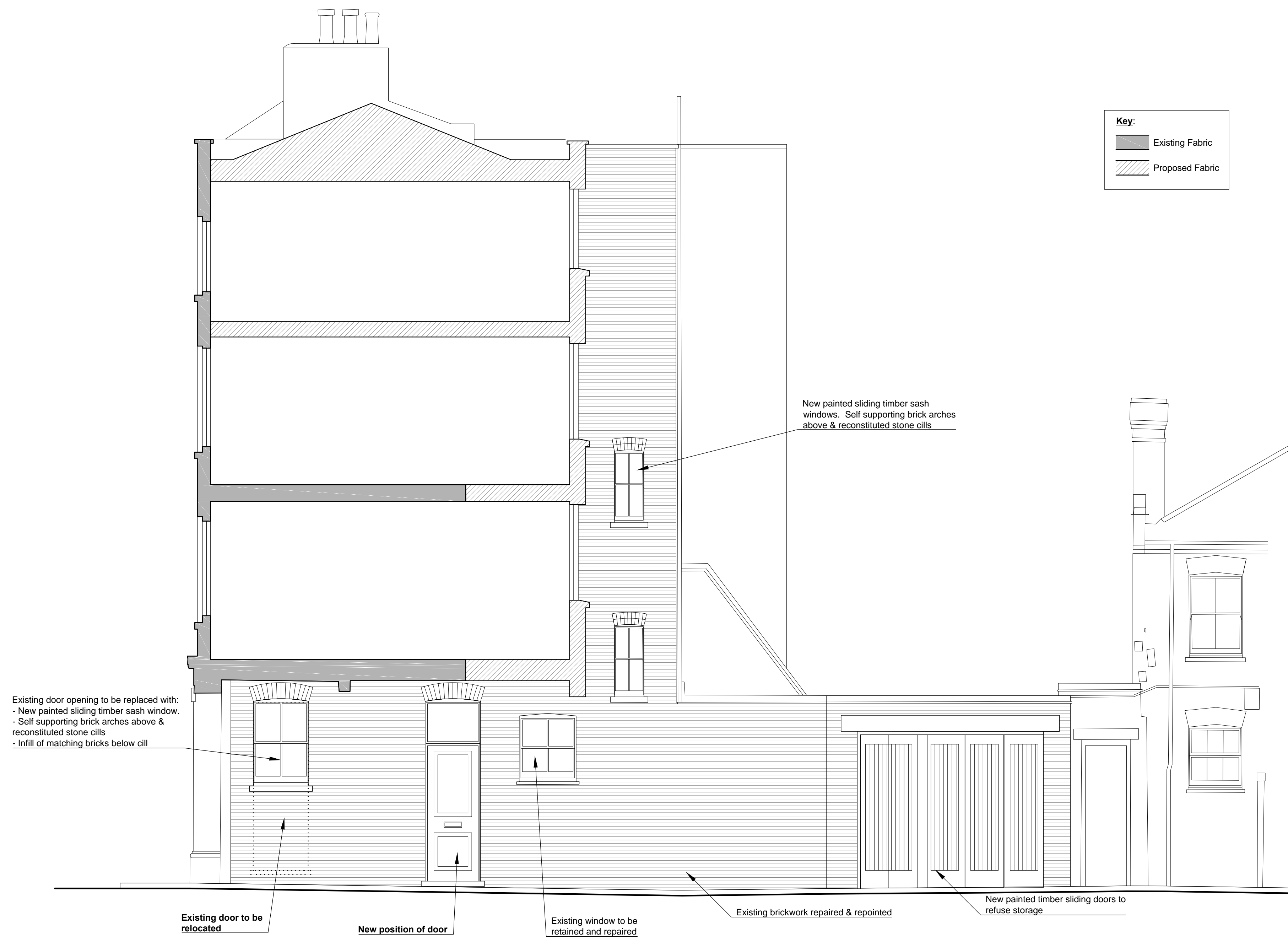
Proposed Section BB Scale 1:50
