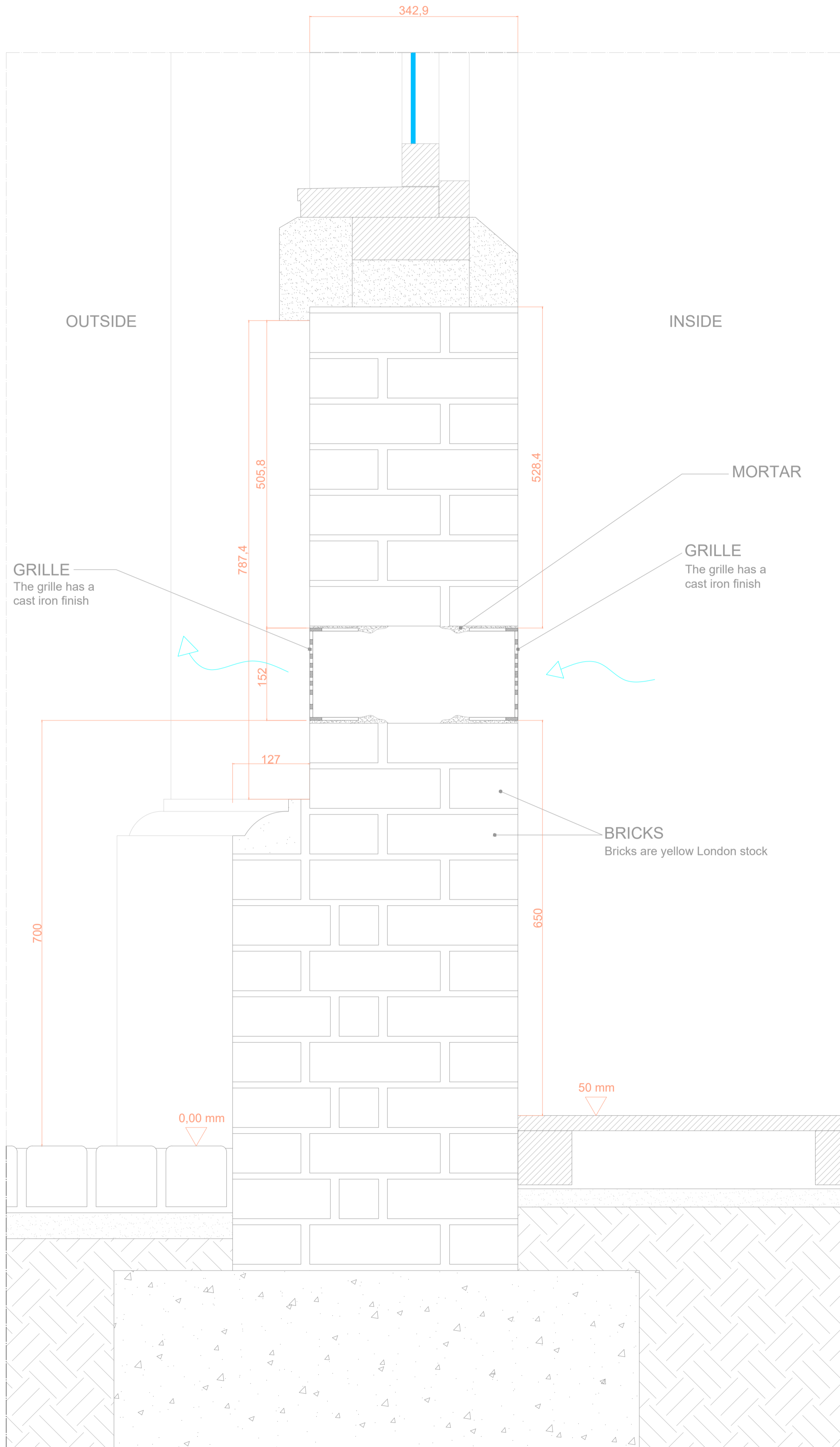
Cross section - Exterior wall - Unit 88
