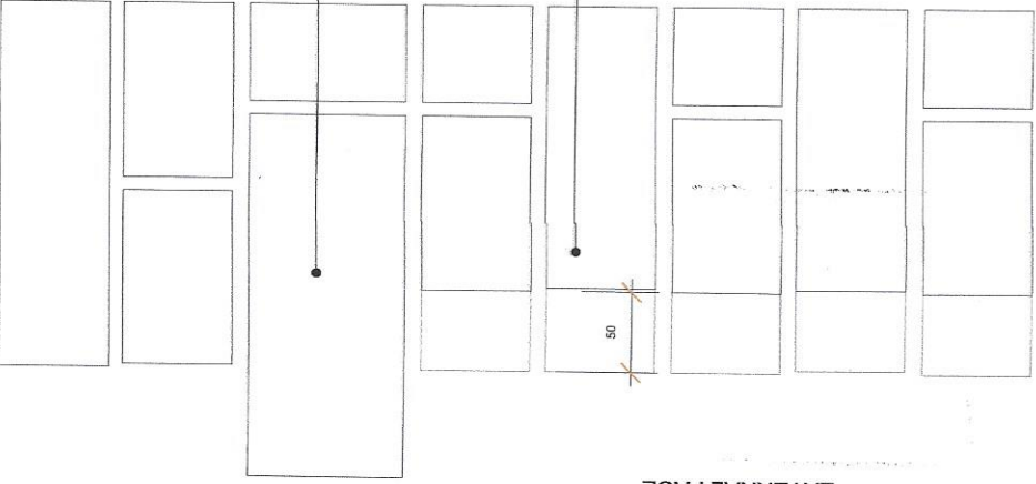
DETAIL-RECESSED BRICK PANELS /D04 Cross section - SCALE 1:5
