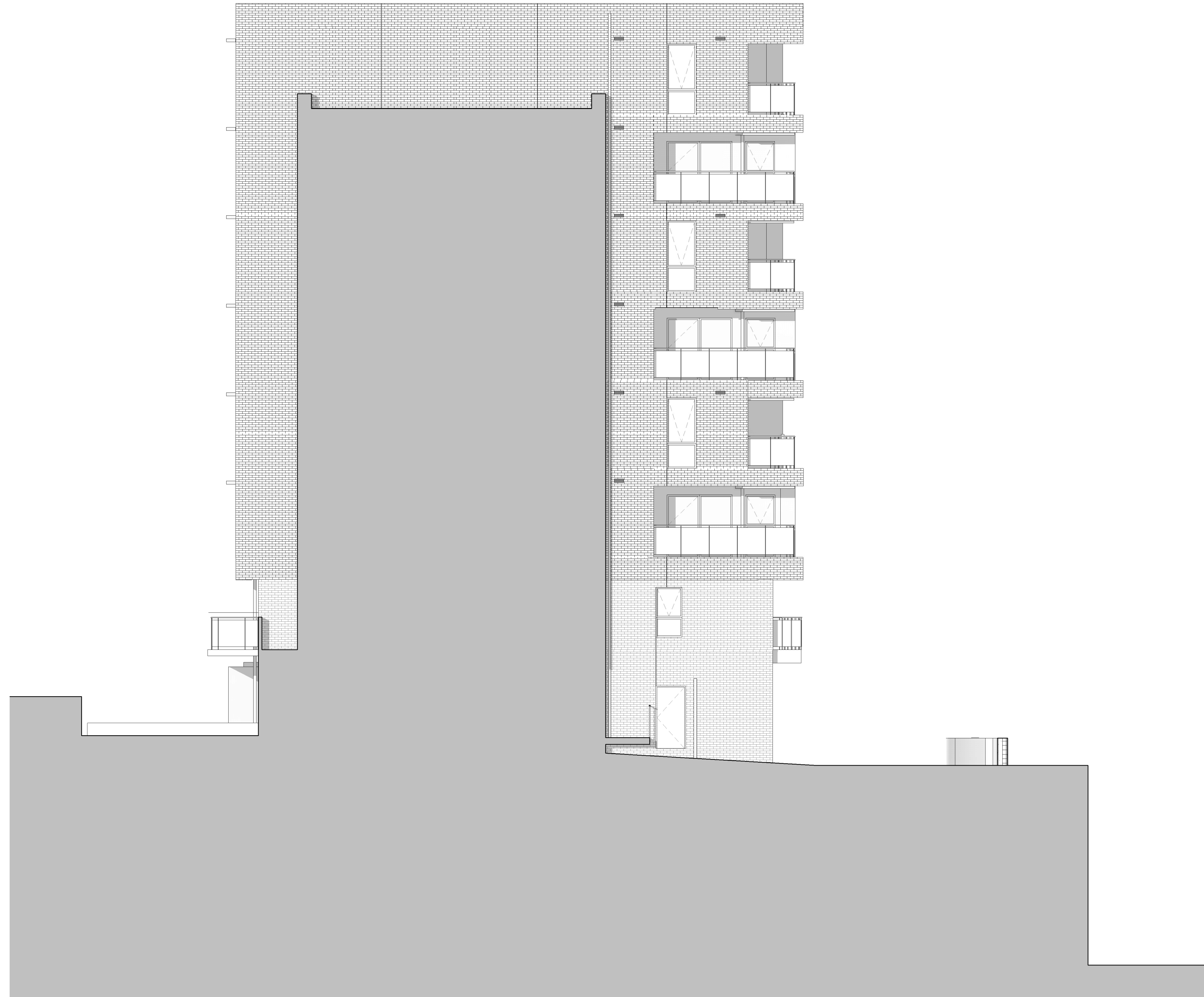
BB 203 Elevation East - Existing 1:100
