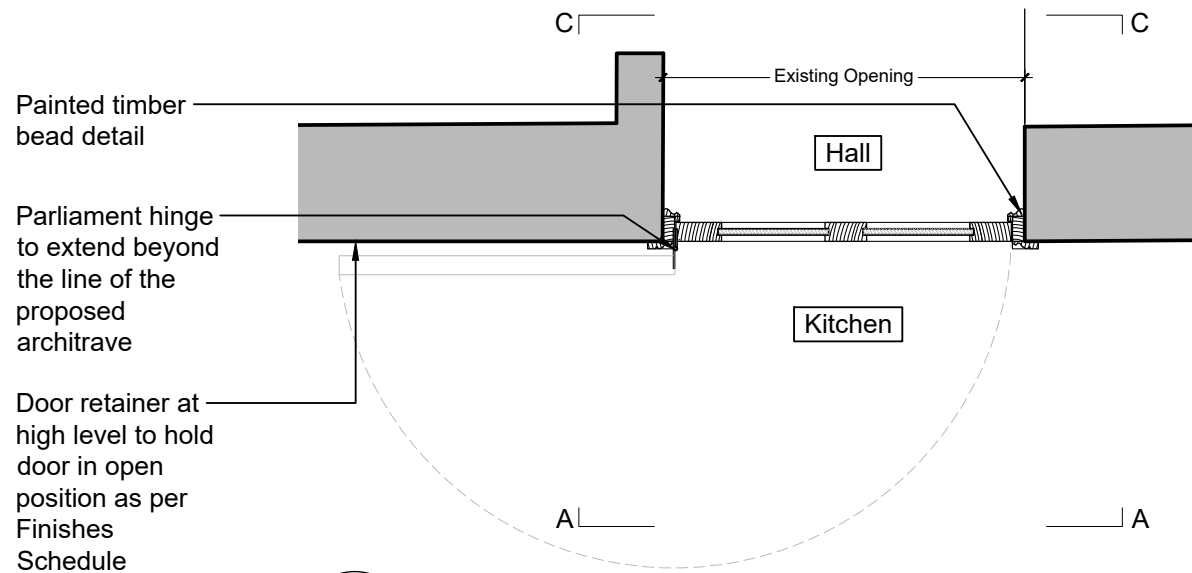
01 Plan D-D 3002 1:20 @ A3
