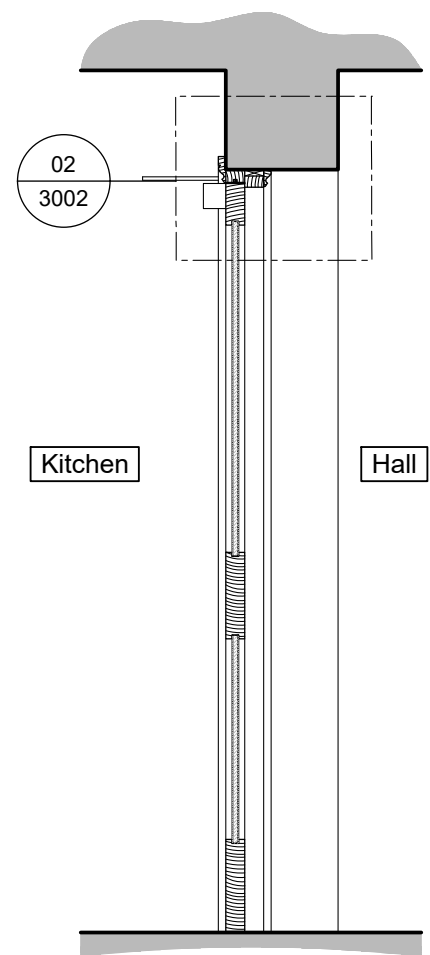
04 Door Section B-B 3002 1:20 @ A3
