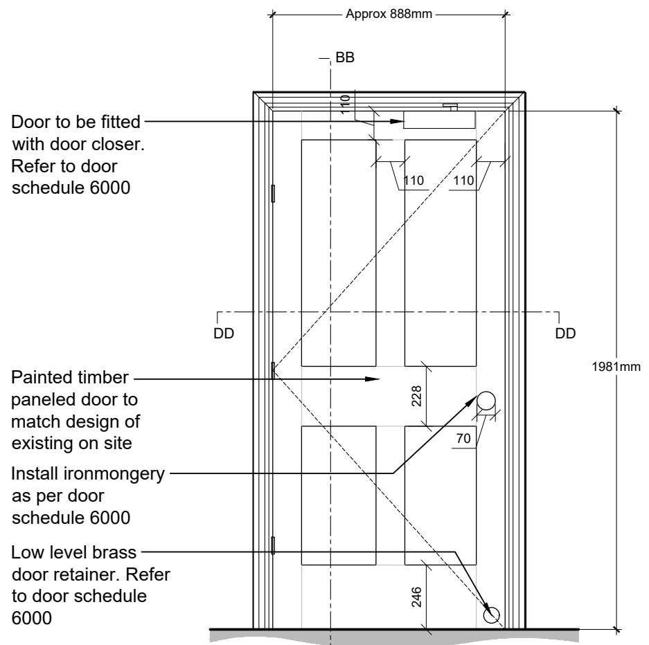
03 Door Elevation AA 3002 1:20 @ A3
