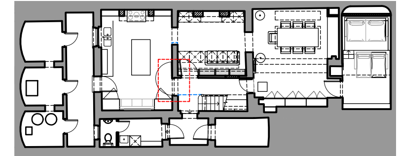
00 Basement Key Plan 3002 1:200 @ A3
