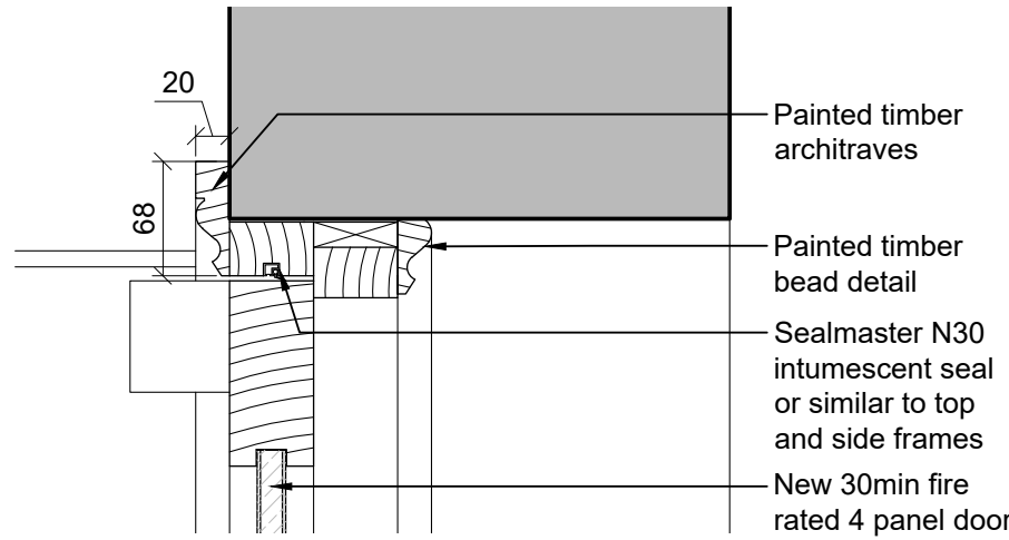
02 Door Head 3002 1:5 @ A3
