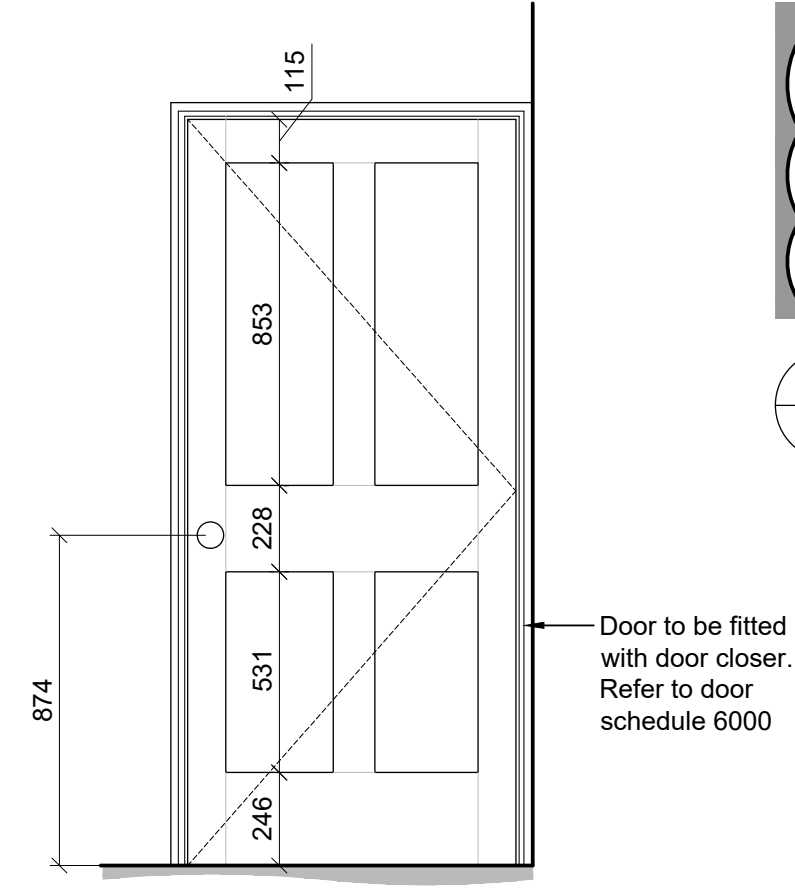
05 Door Elevation C-C 3002 1:20 @ A3
