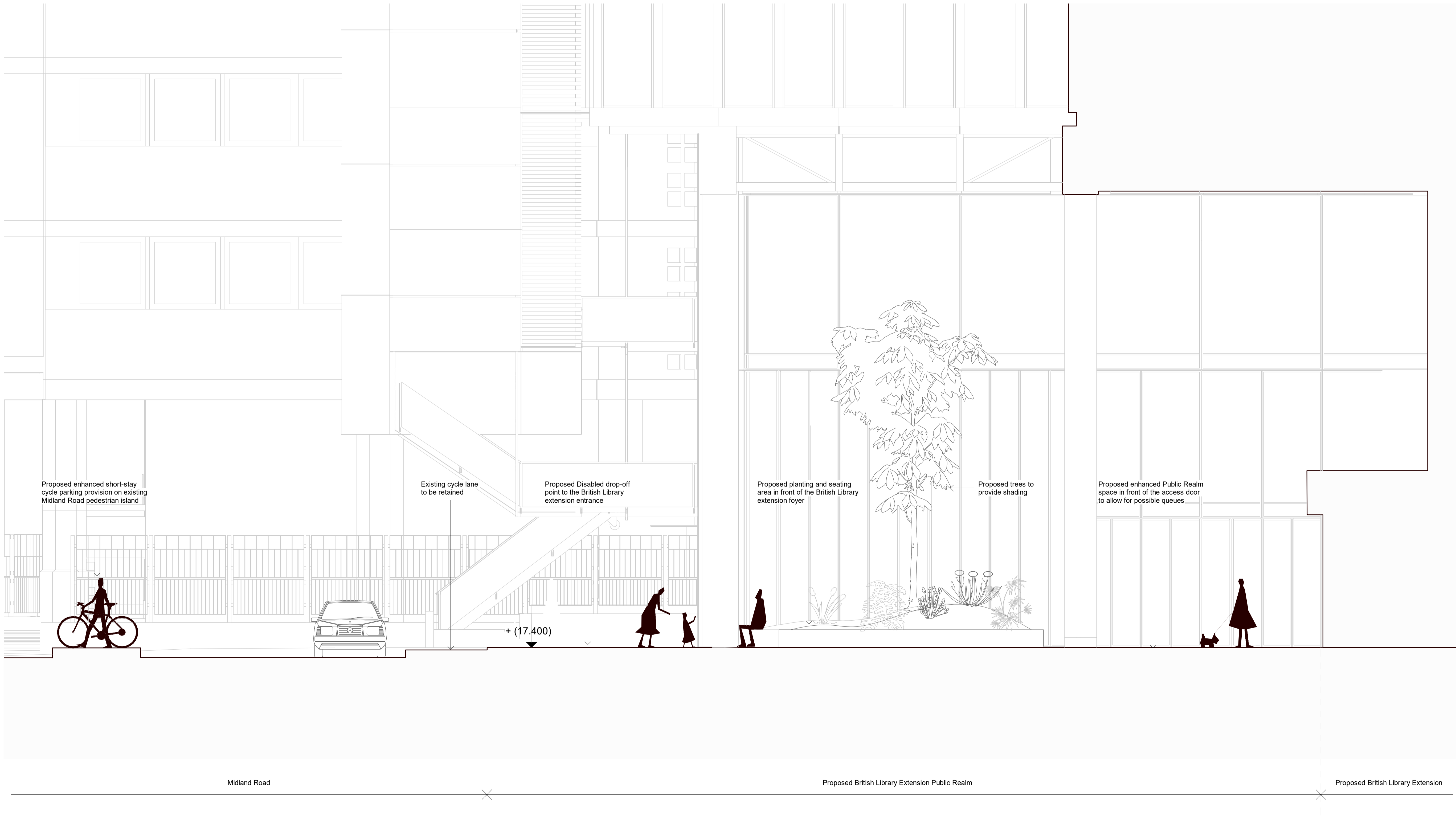
PROPOSED SITE SECTION A-A - MIDLAND ROAD Scale 1:50
