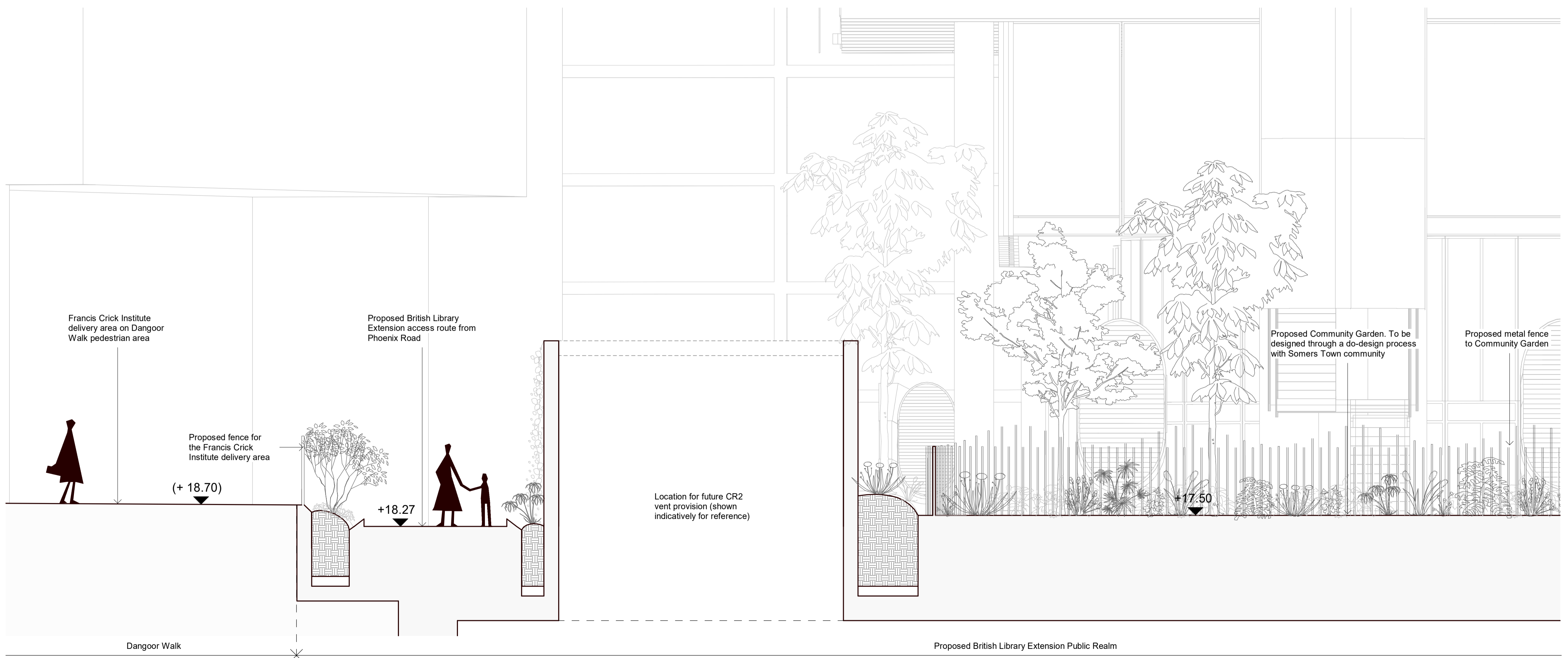
PROPOSED SITE SECTION E-E - DANGOOR WALK Scale 1:50
