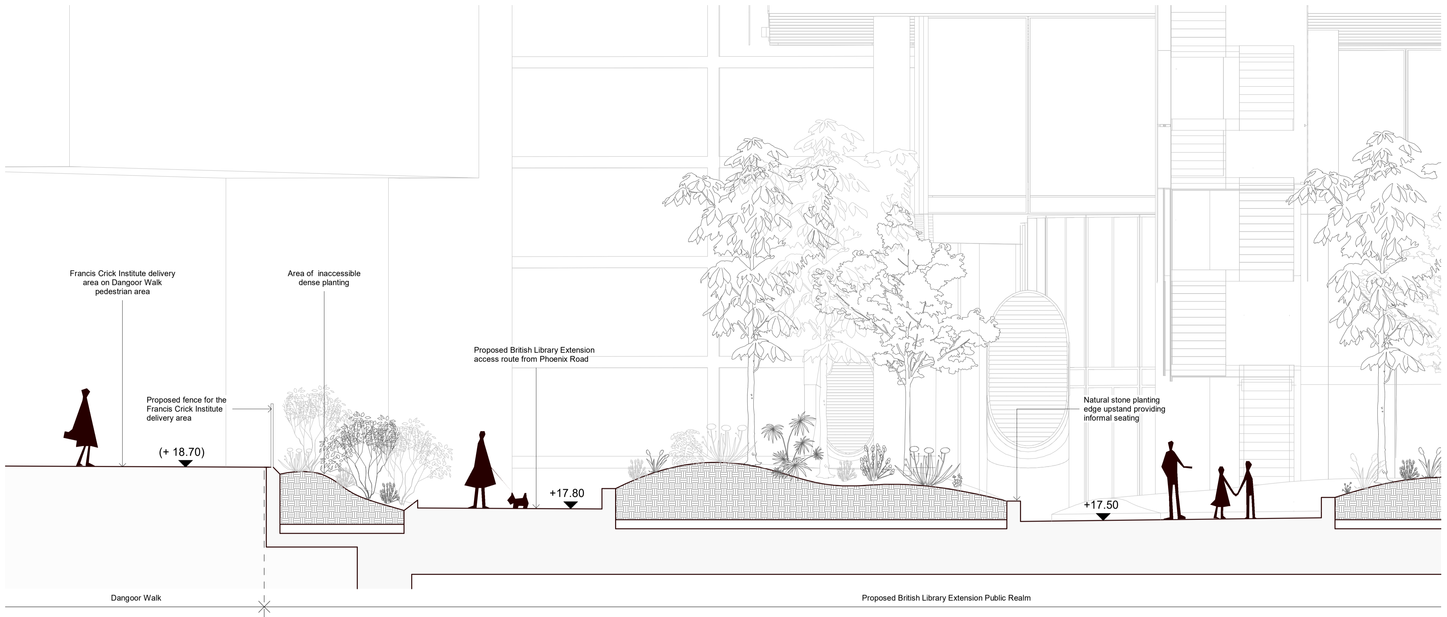
PROPOSED SITE SECTION D-D - DANGOOR WALK Scale 1:50
