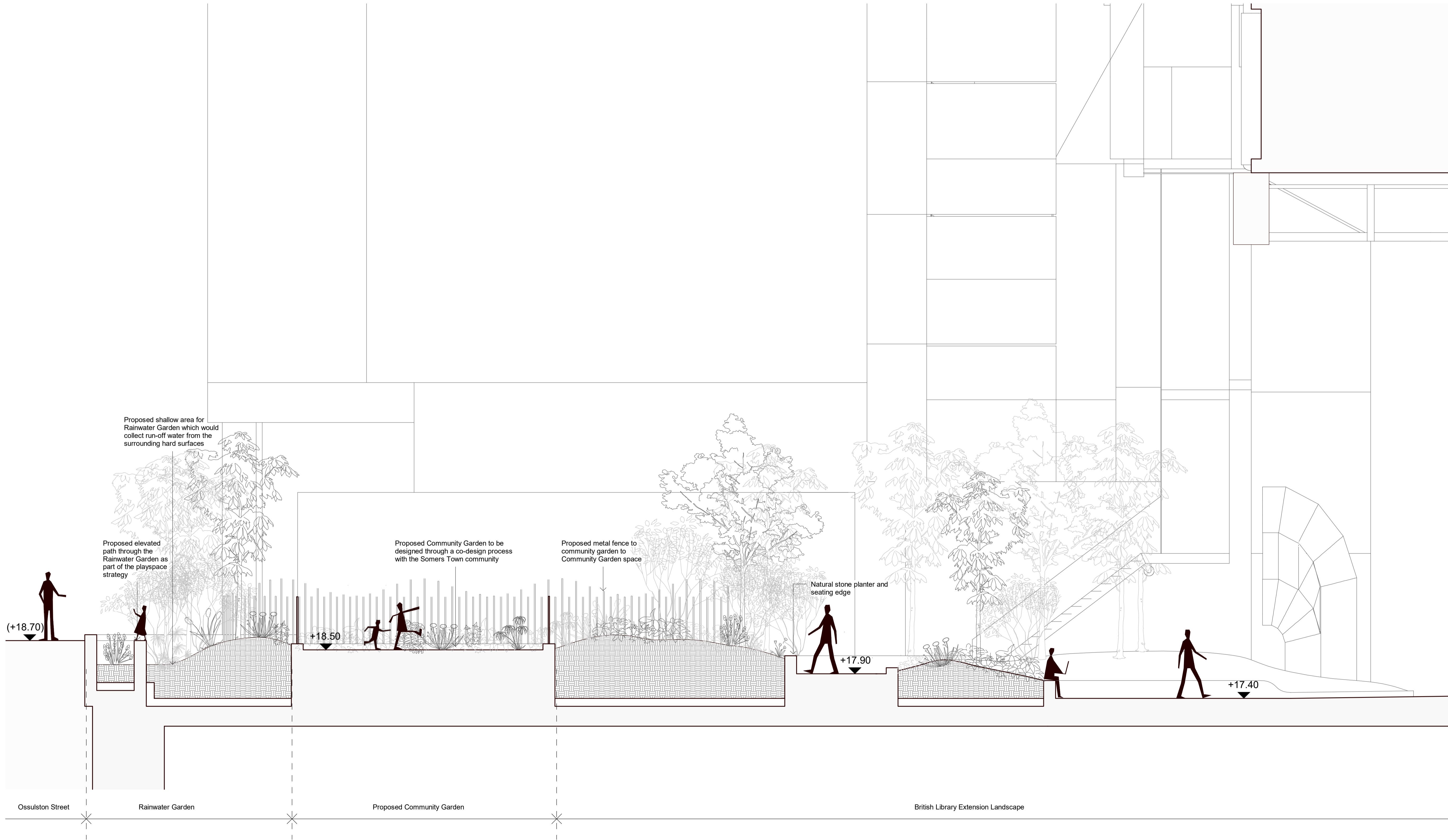
PROPOSED SITE SECTION H-H - OSSULSTON STREET COMMUNITY GARDEN Scale 1:50
