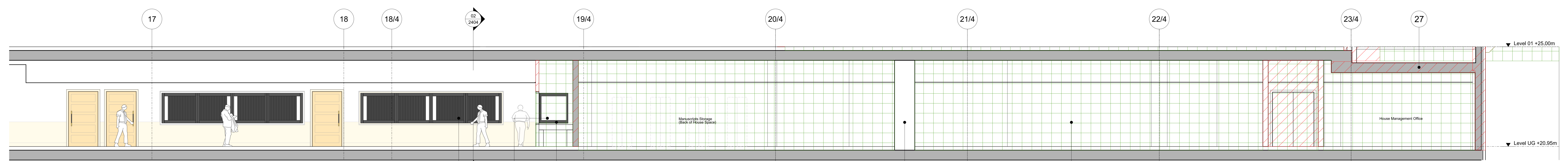
02 Existing Level UG Demolition / Alteration Elevation Looking West 1:50
