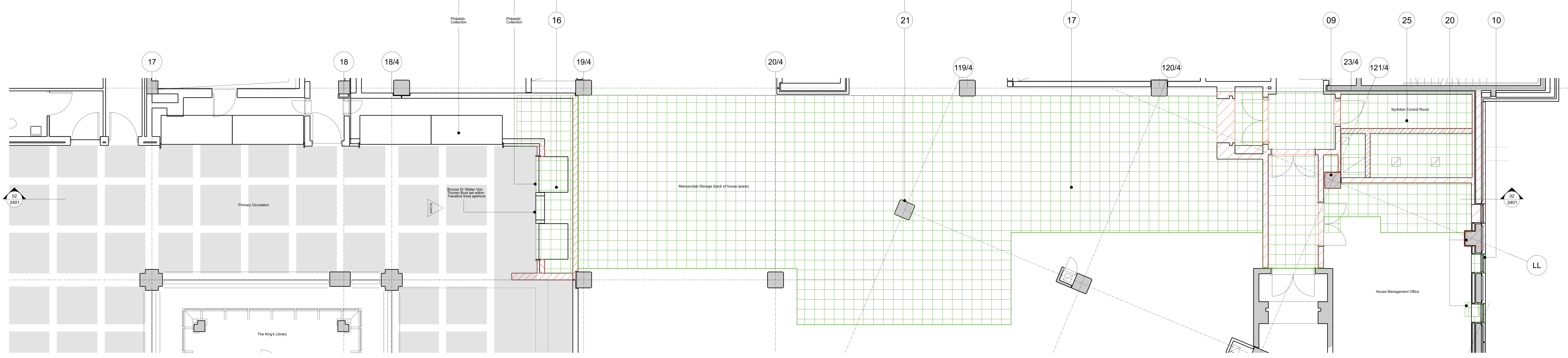
01 Existing Level UG Demolition / Alteration Plan 1:50
