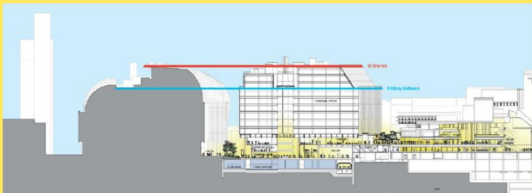
Cross section showing heights of the extension and internal foyer area
