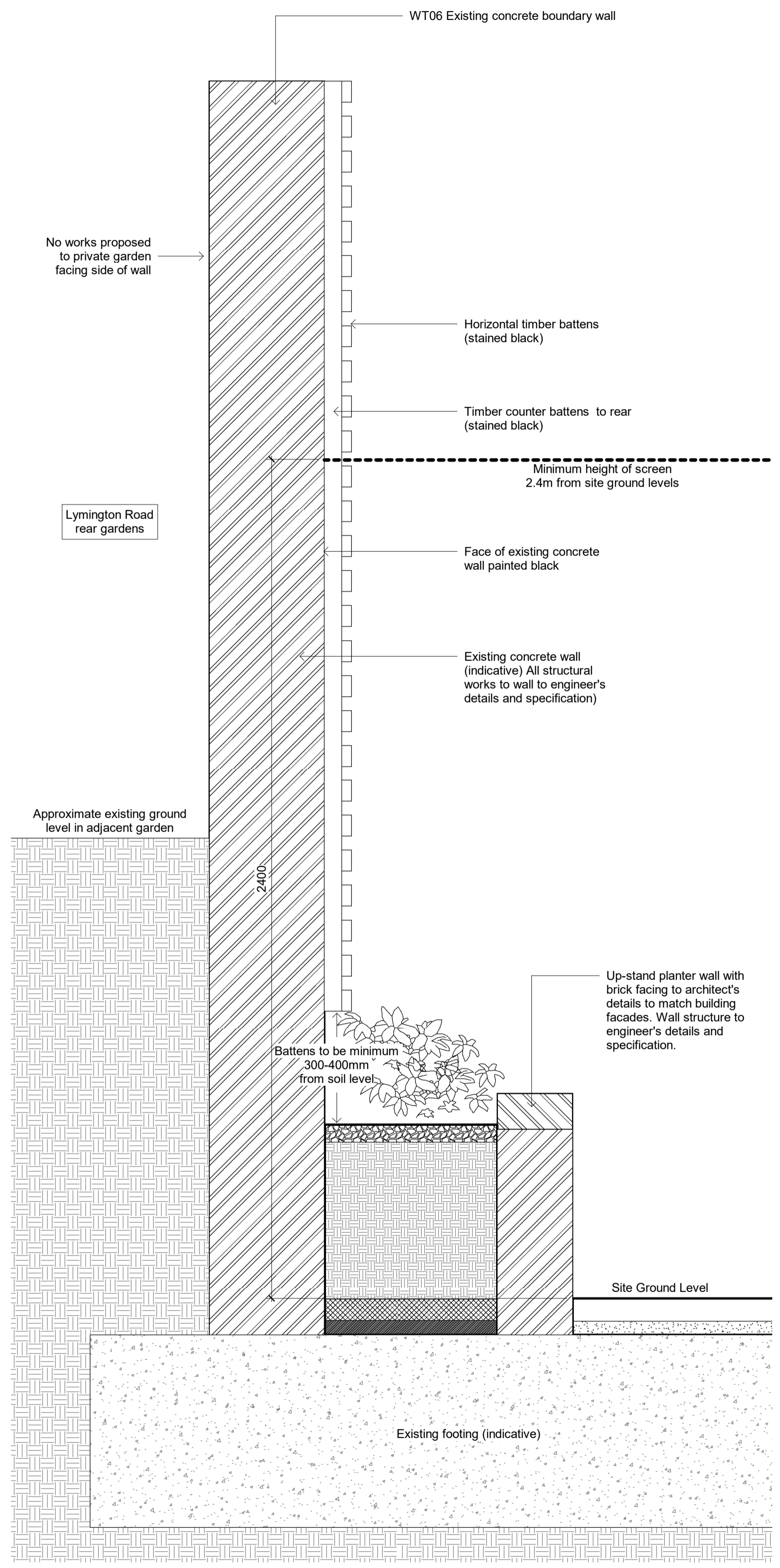
2 Northern Boundary Wall Typical Section Through Wall Type 06 With Planter Scale 1 : 10
