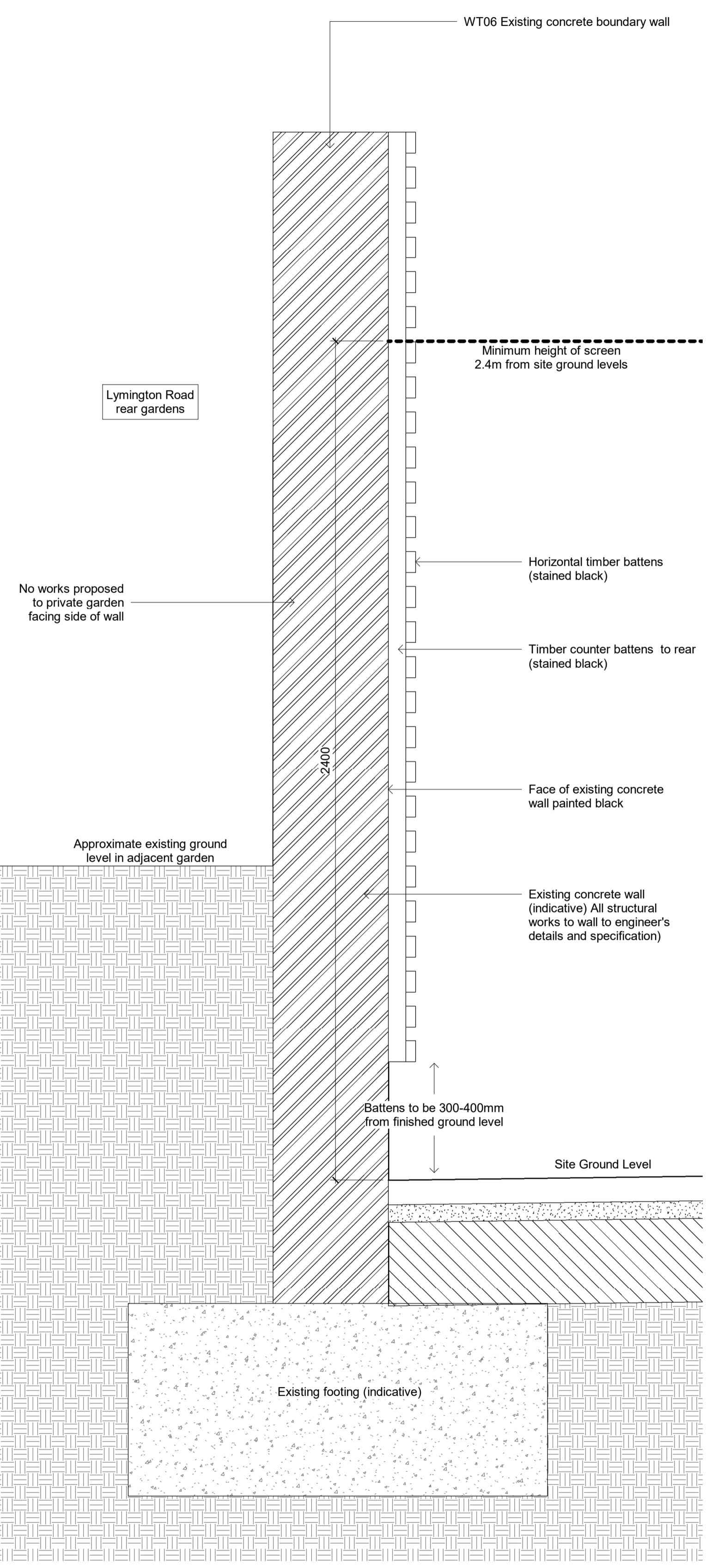
1 Northern Boundary Wall Typical Section Through Wall Type 06 Without Planter Scale 1 : 10
