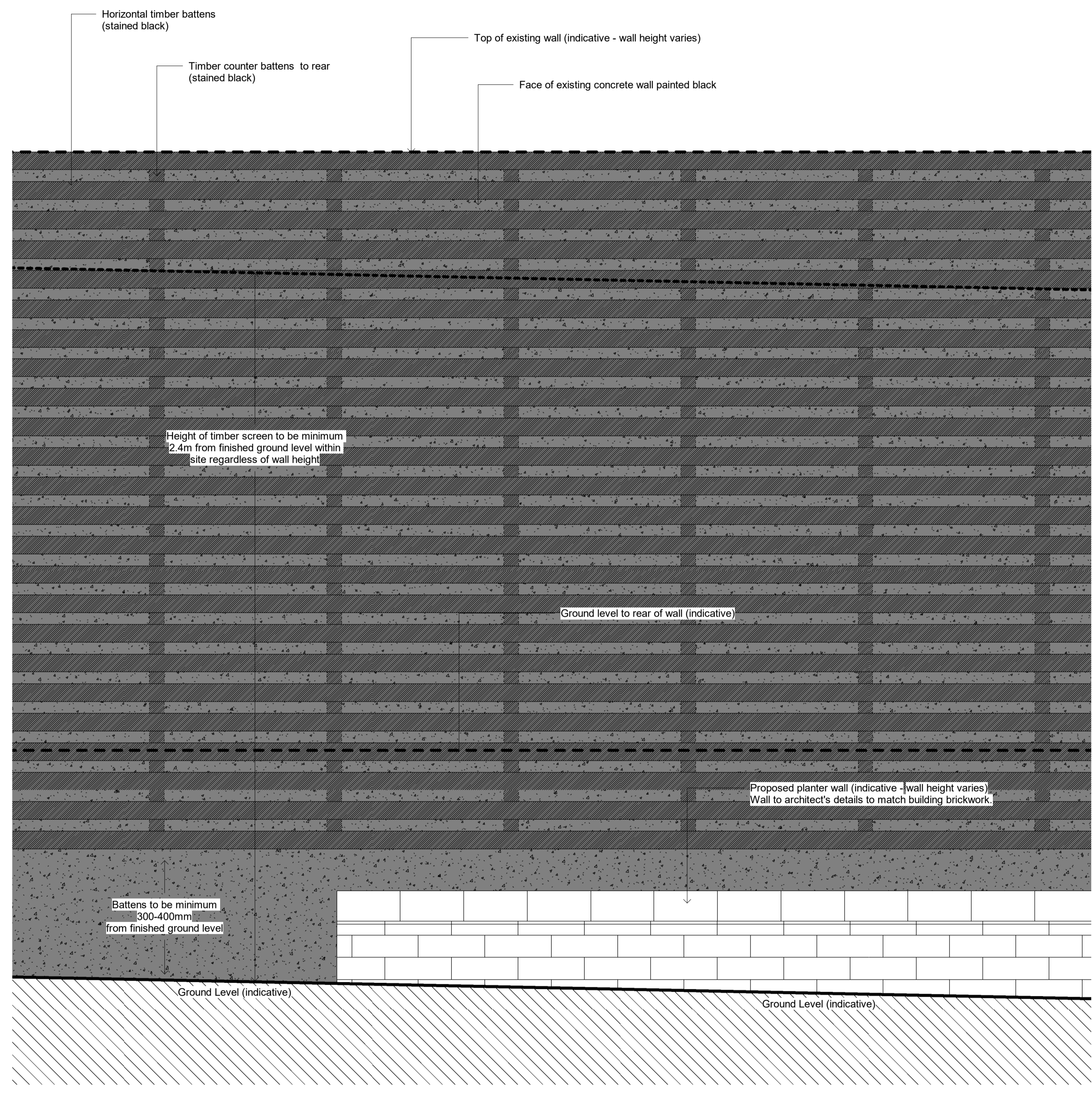
3 Northern Boundary Wall - Typical Elevation Scale 1 : 10
