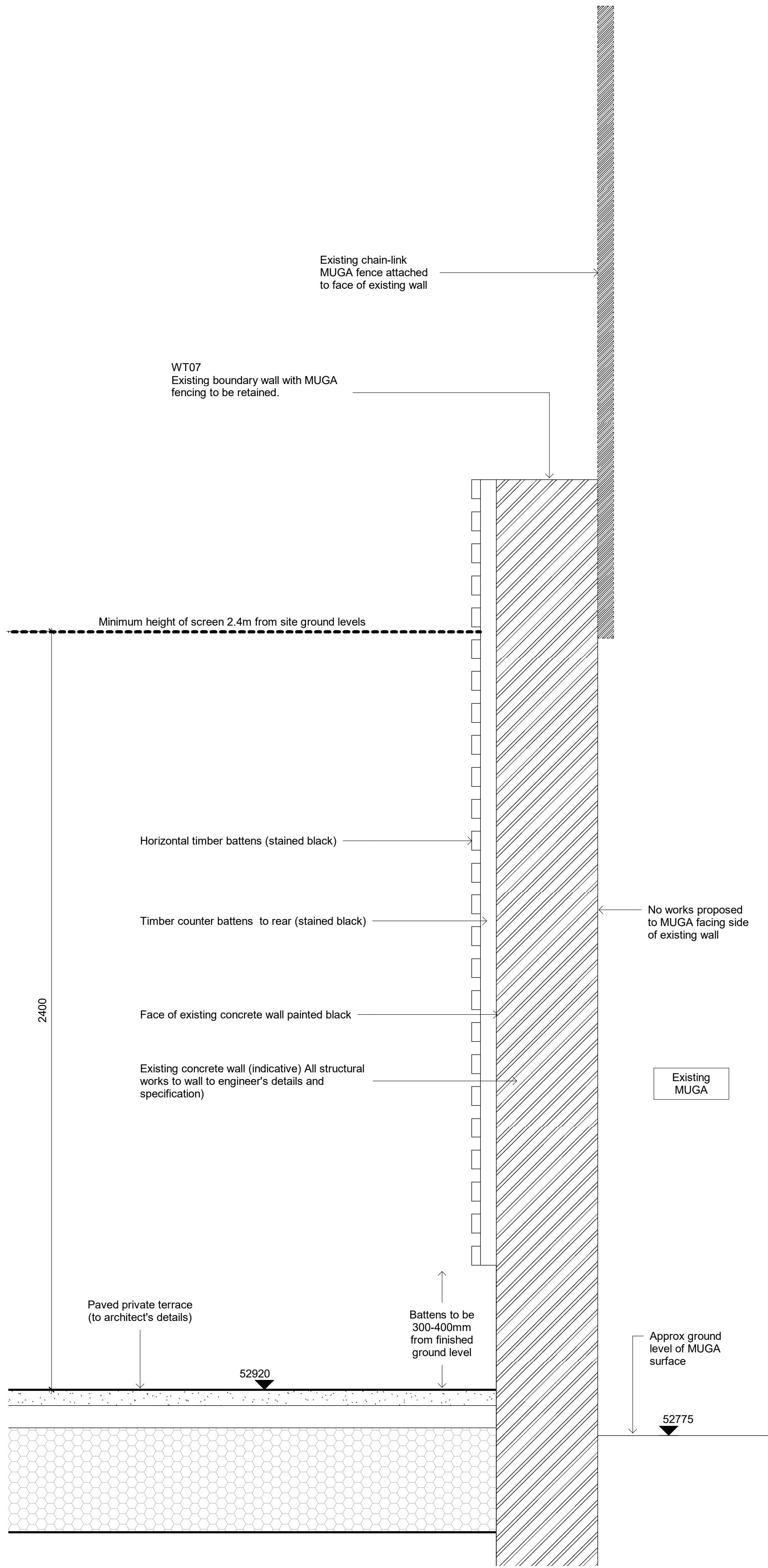
1 Eastern Boundary Wall - Typical Section Scale 1 : 10
