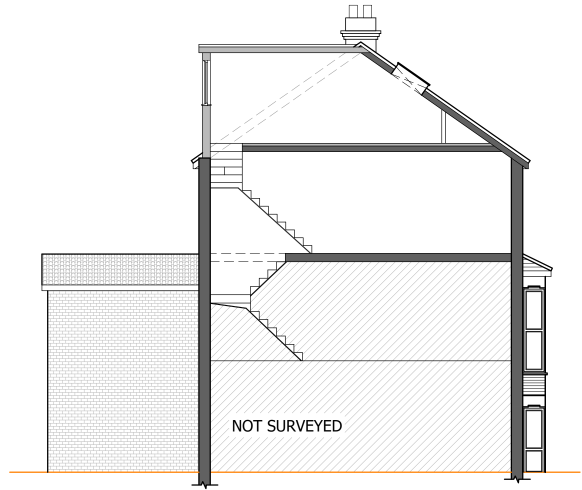
PROPOSED SECTION
