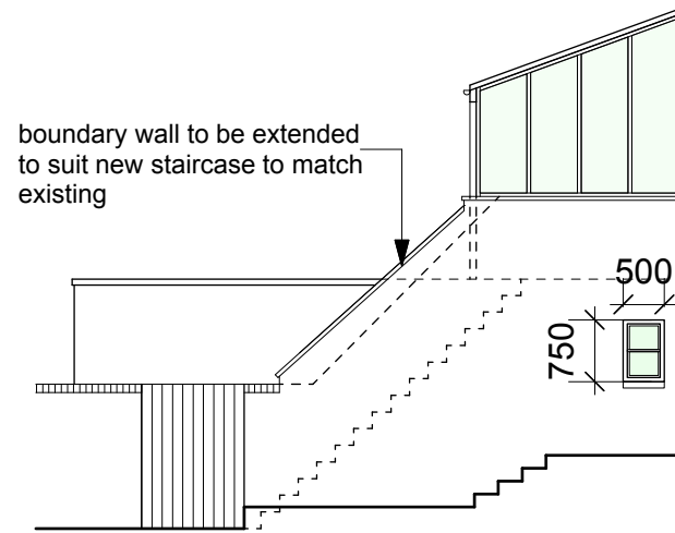
Proposed Side Elevation (Side Passage)
