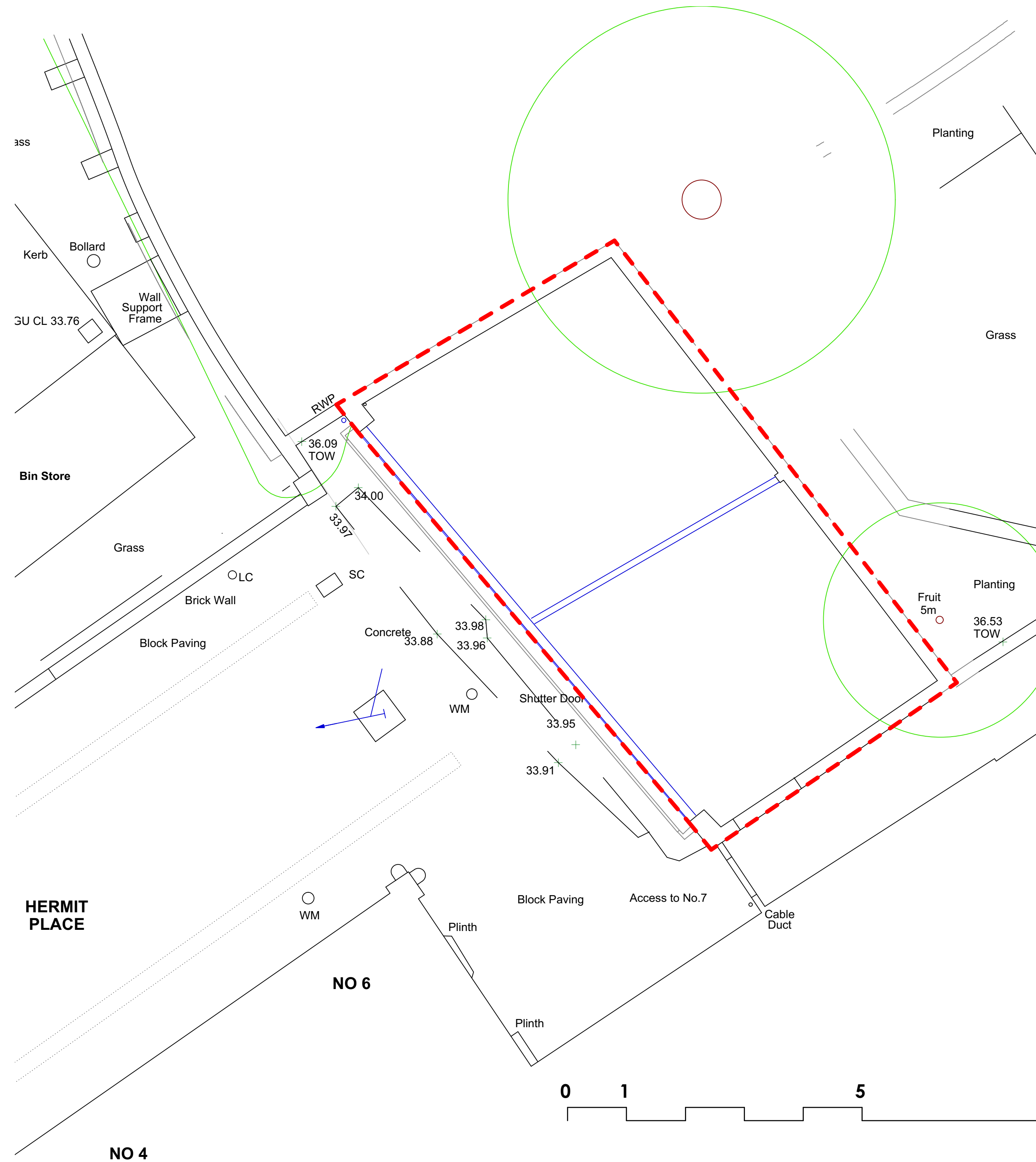
LOCATION PLAN
