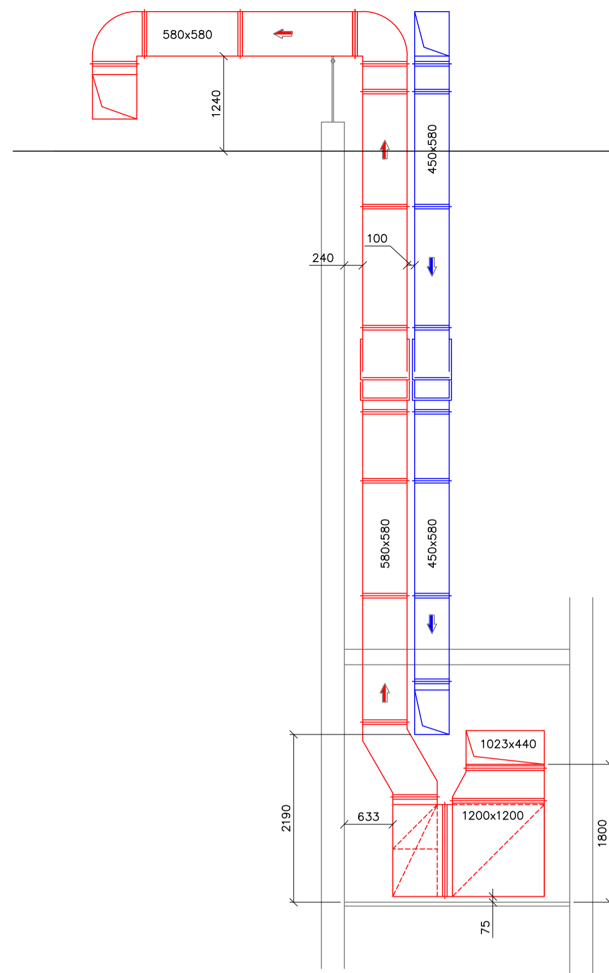
SECTION AA SCALE 1:50
