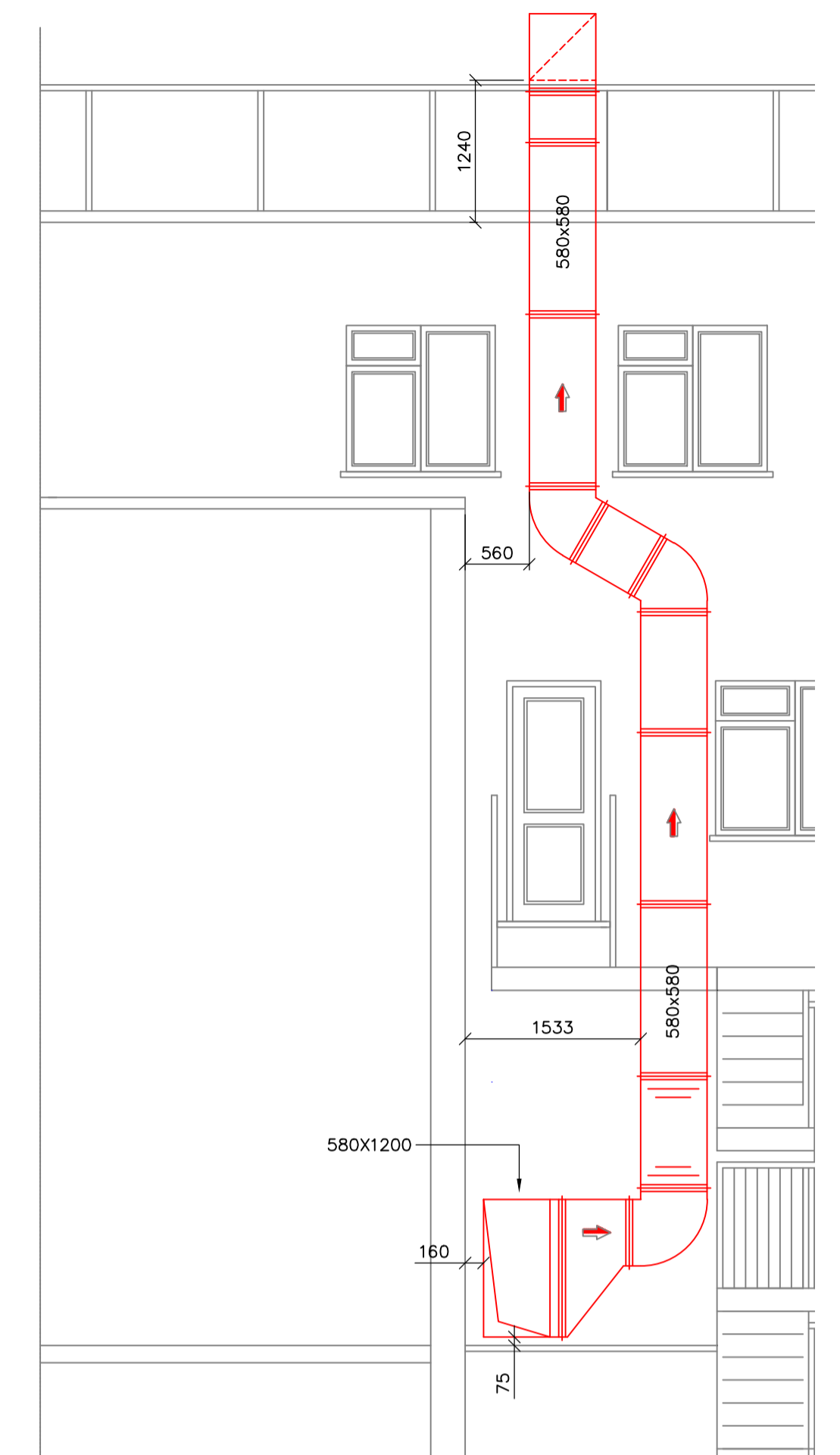
SECTION CC SCALE 1:50
