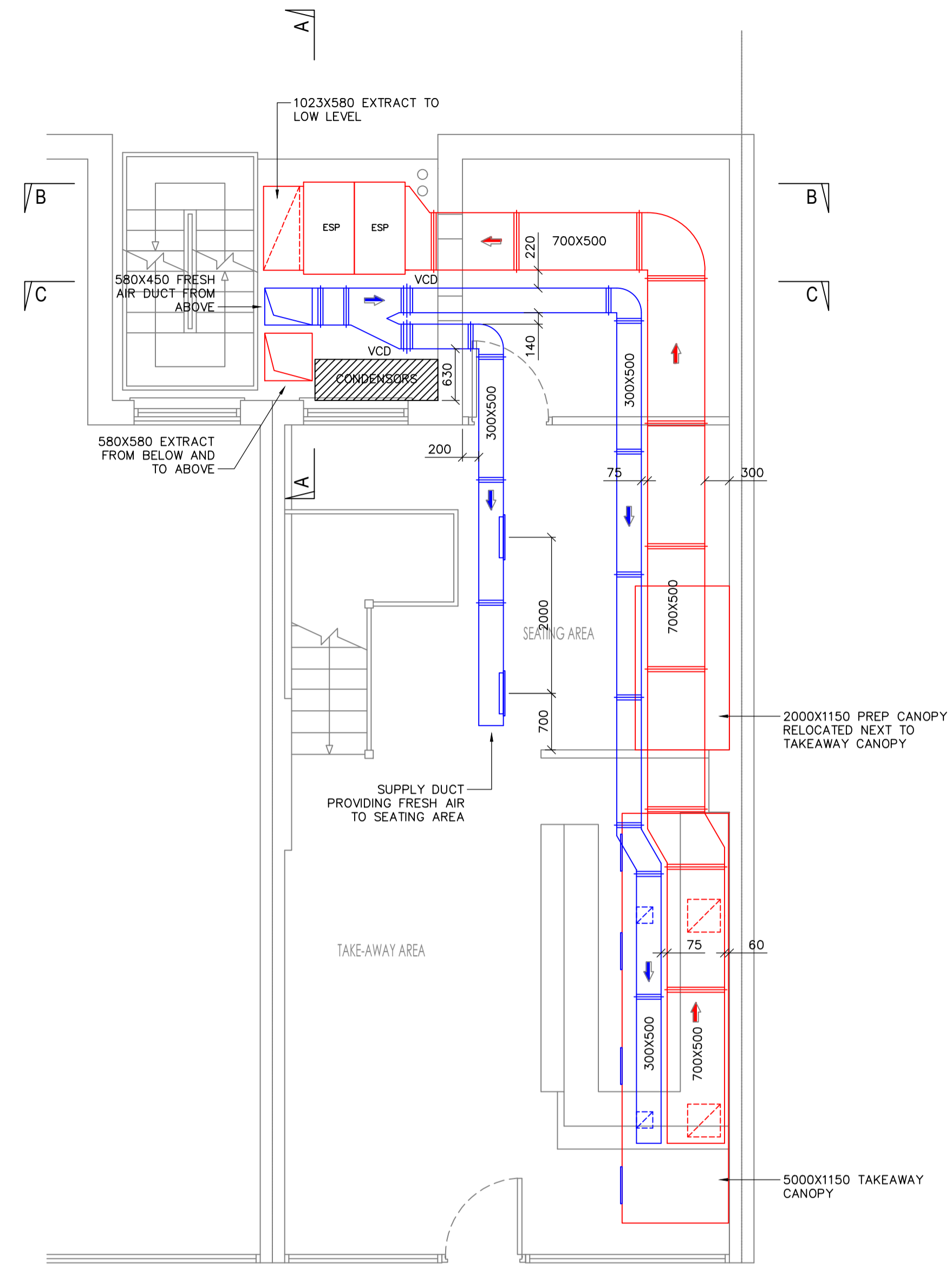
GROUND FLOOR HIGH LEVEL SCALE 1:50
