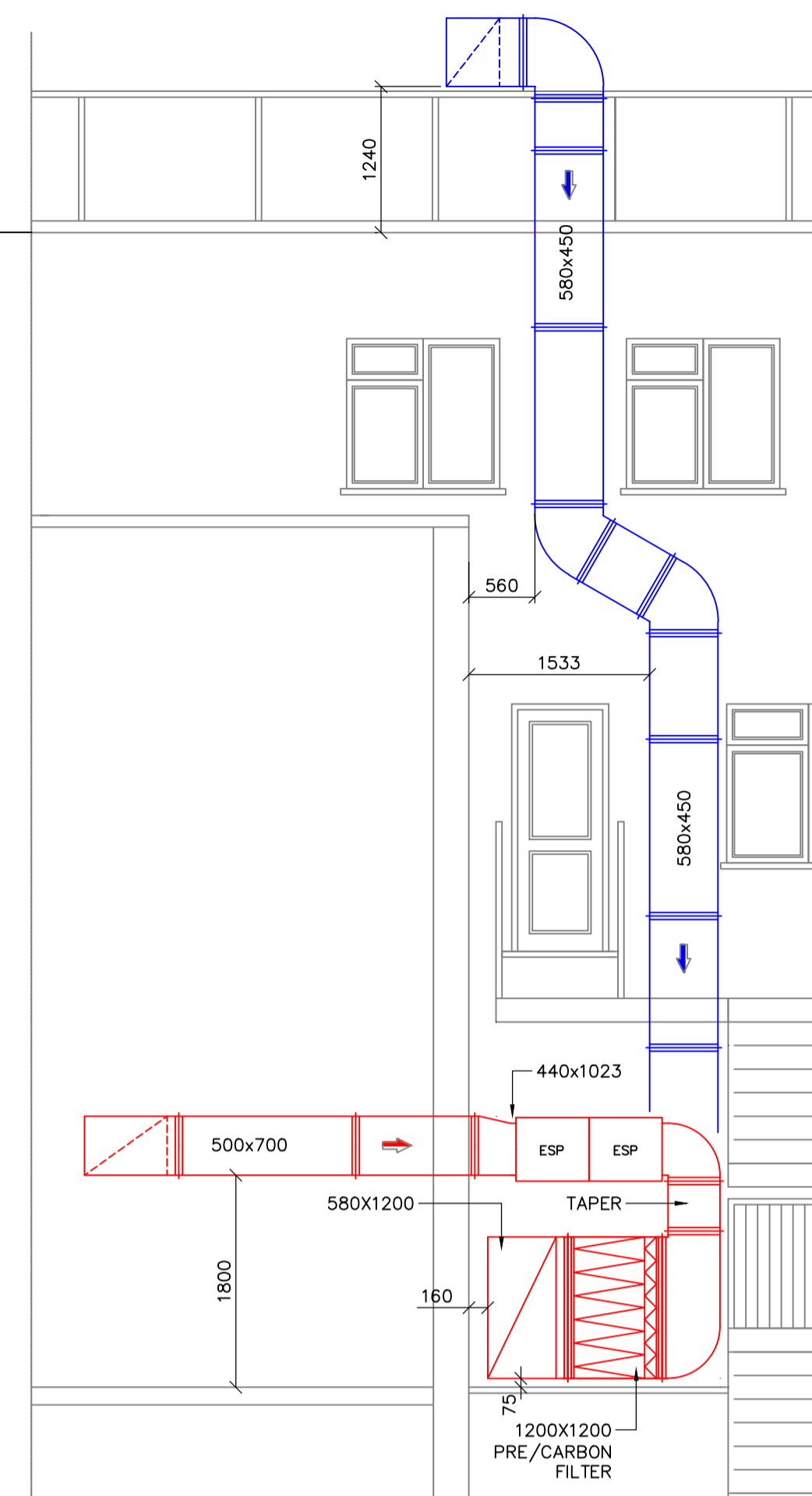
SECTION BB SCALE 1:50
