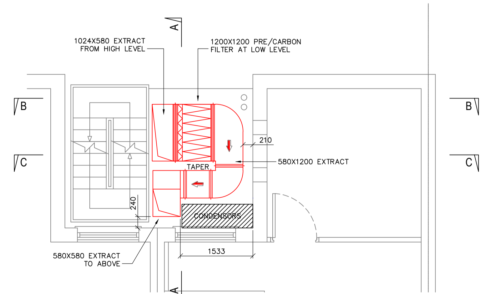
GROUND FLOOR LOW LEVEL SCALE 1:50
