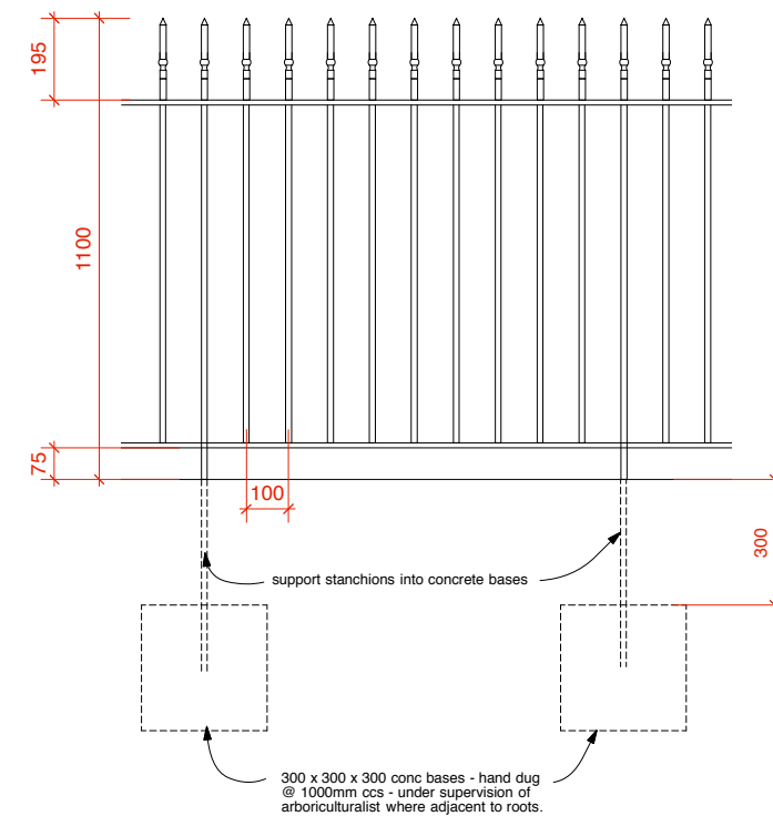
RAILINGS DETAIL
