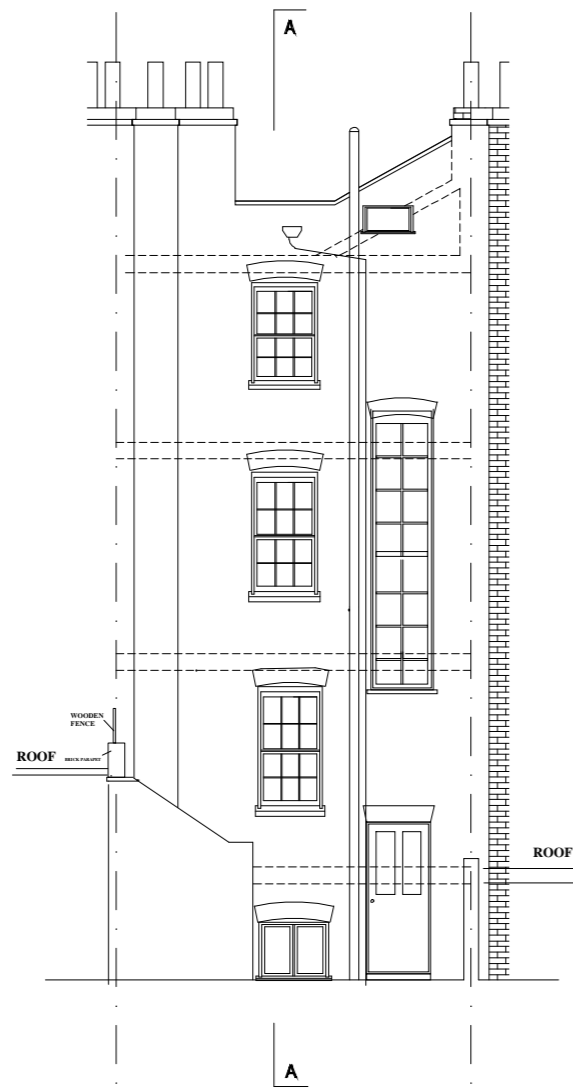
REAR ELEVATION
