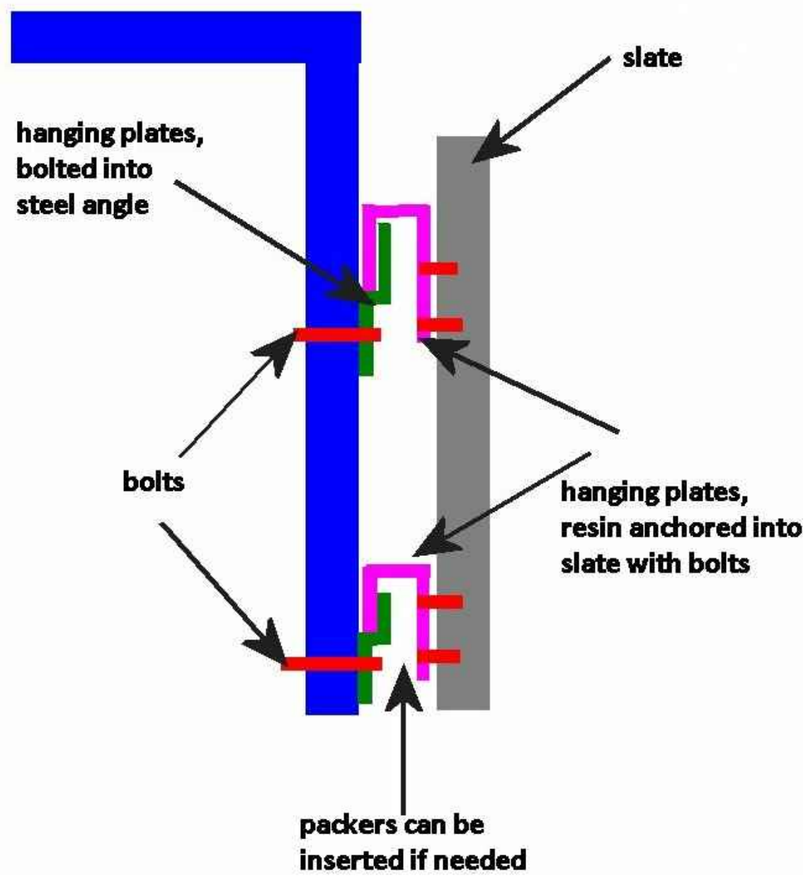
Figure 2: ABA's sketch proposal for hanging slate inscription (not to scale).
