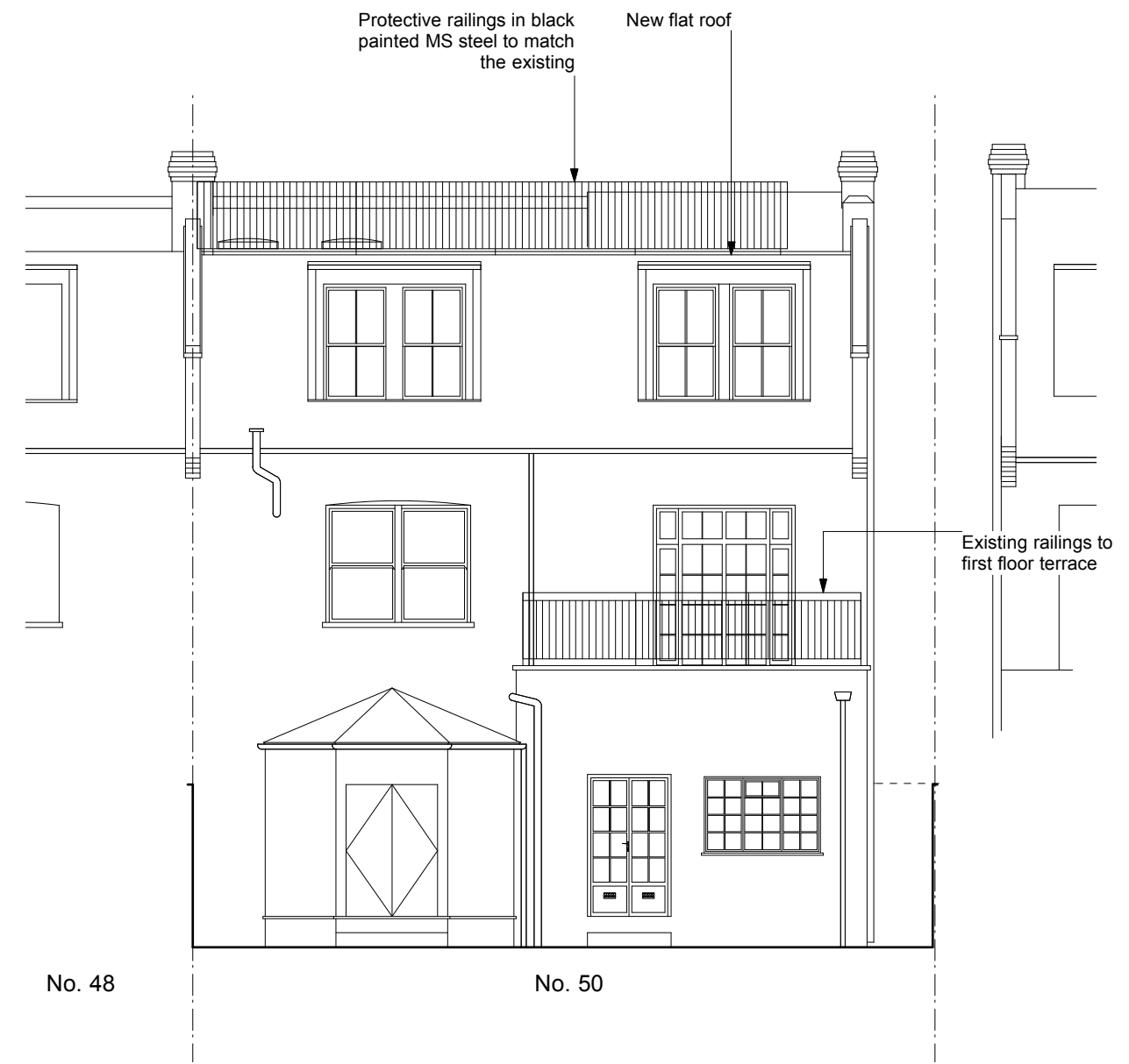
2 REAR ELEVATION
