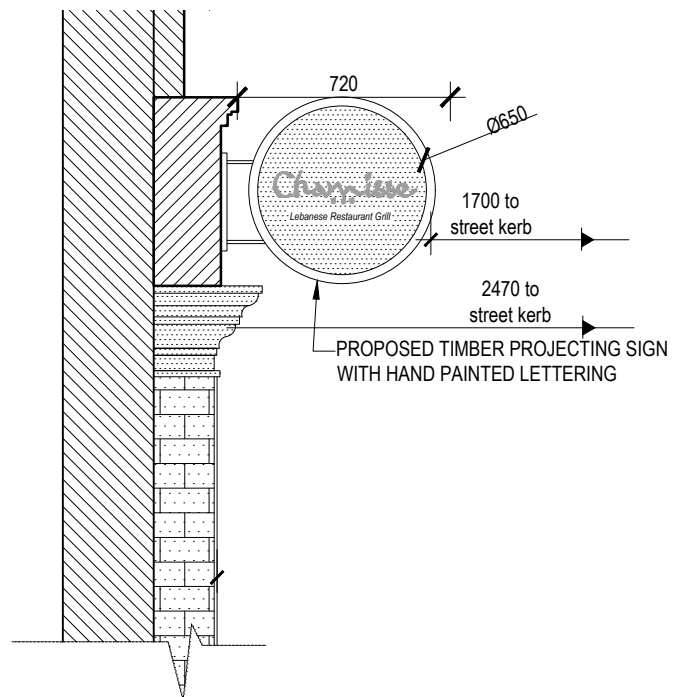
SECTION A-A THROUGH SIDE SIGN
