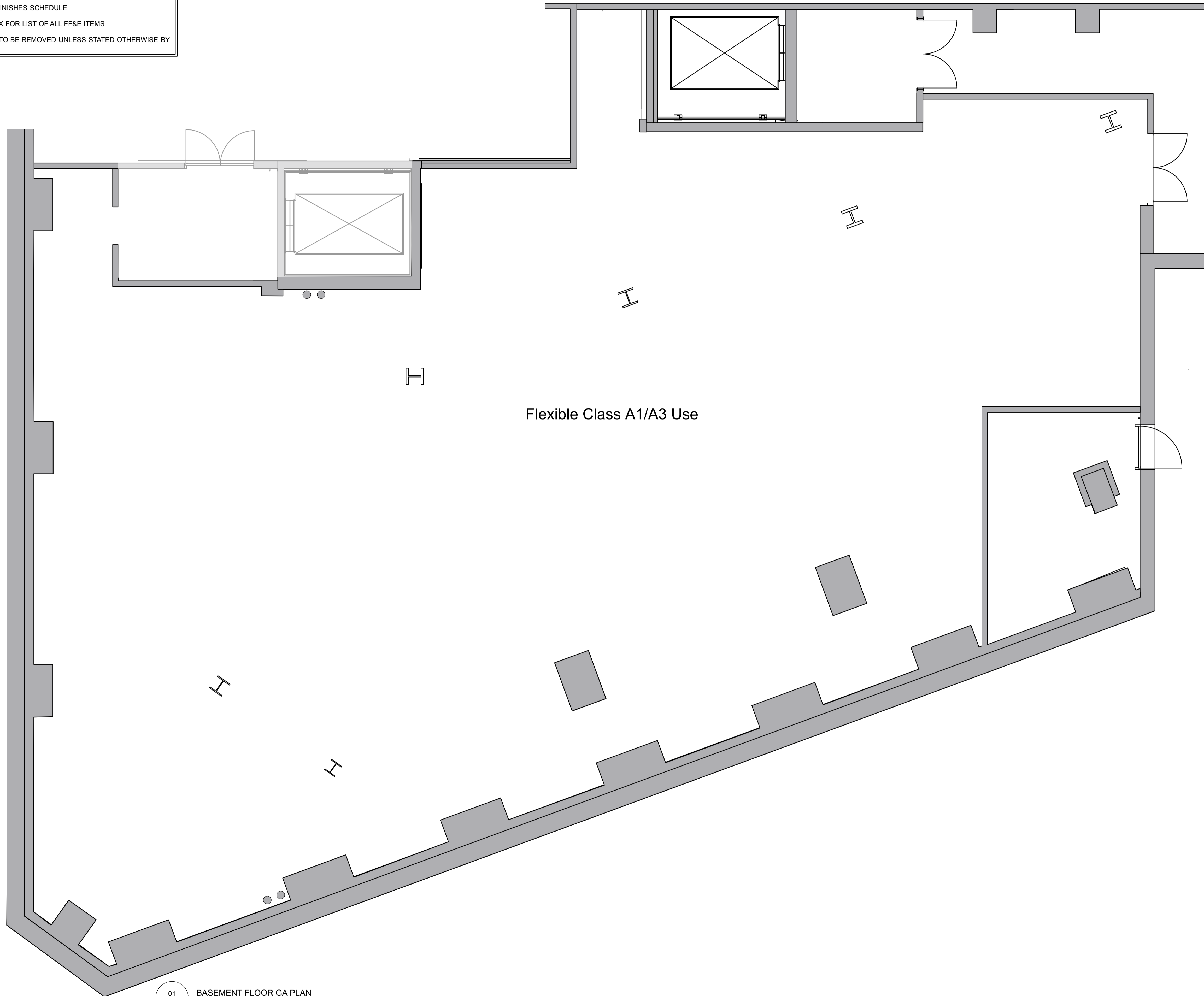
01 PL-B-01 BASEMENT FLOOR GA PLAN Scale: 1:50
