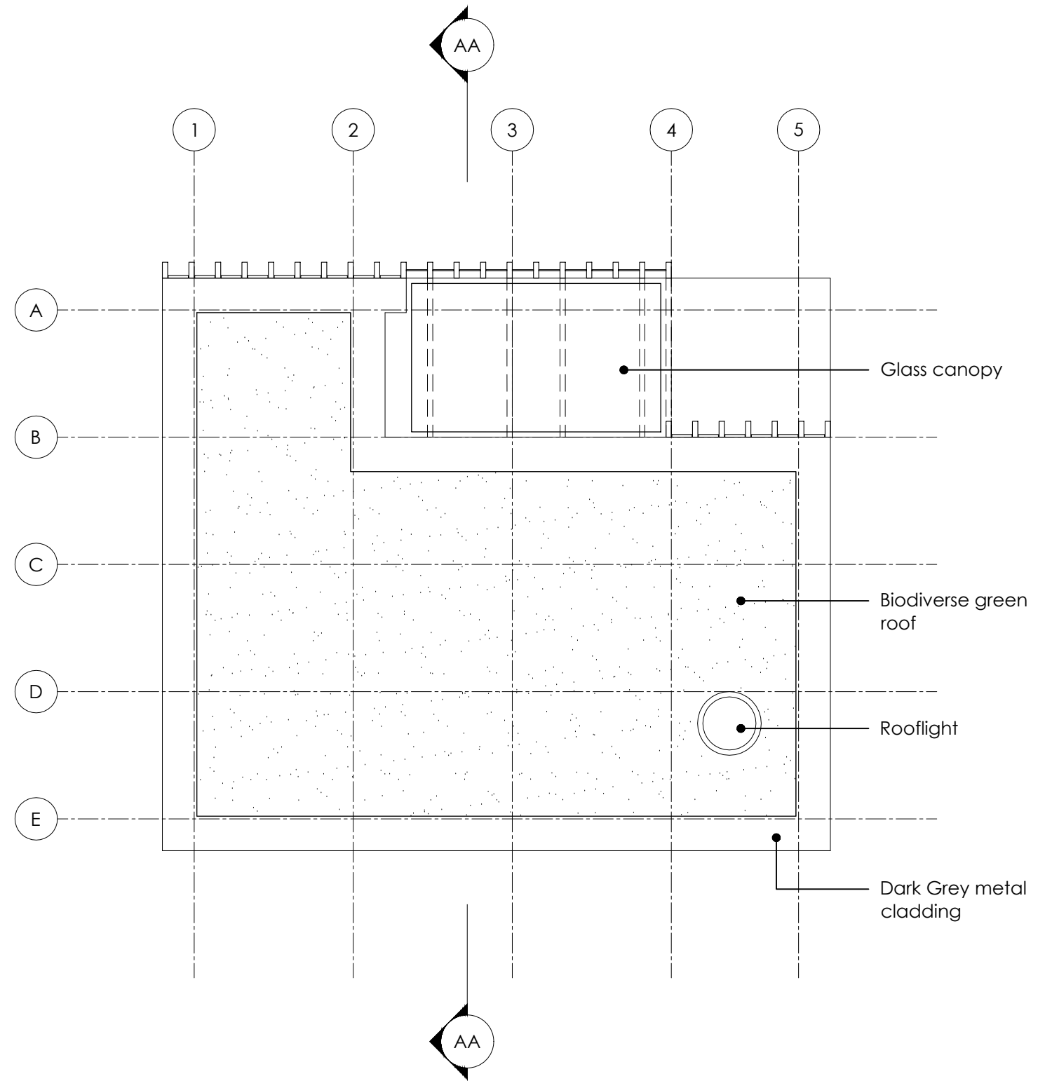
2 Roof Plan
