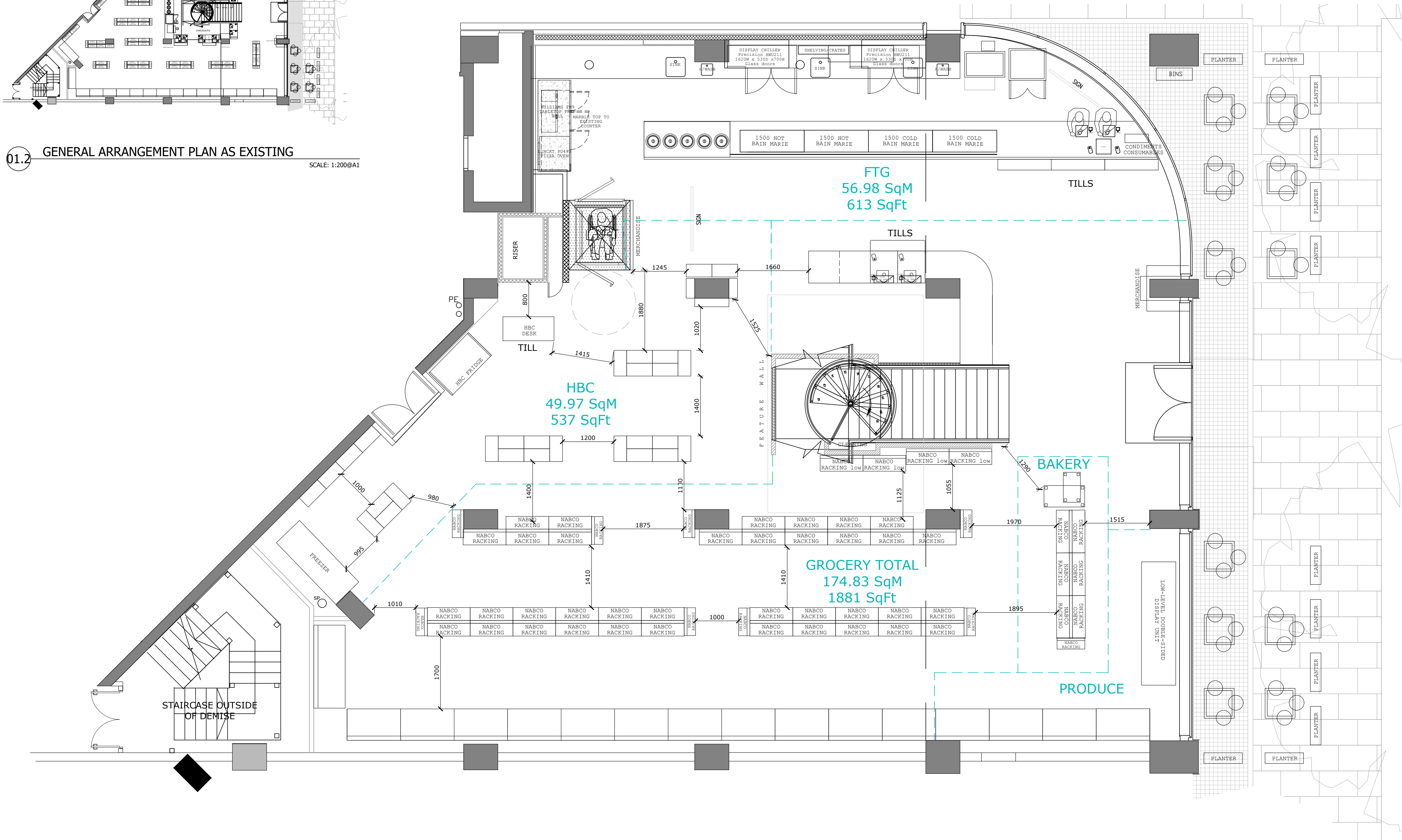
01.1 GENERAL ARRANGEMENT PLAN AS PROPOSED
