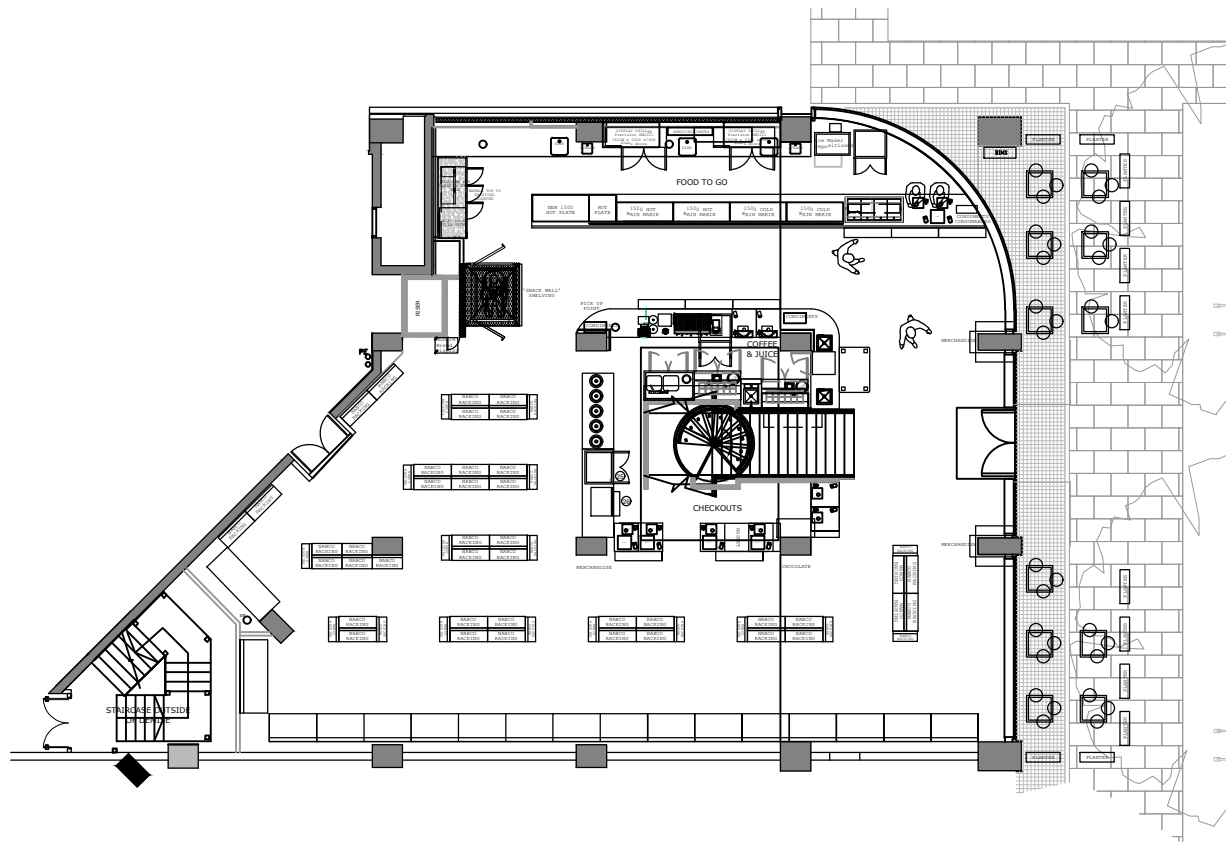
01.2 GENERAL ARRANGEMENT PLAN AS EXISTING
