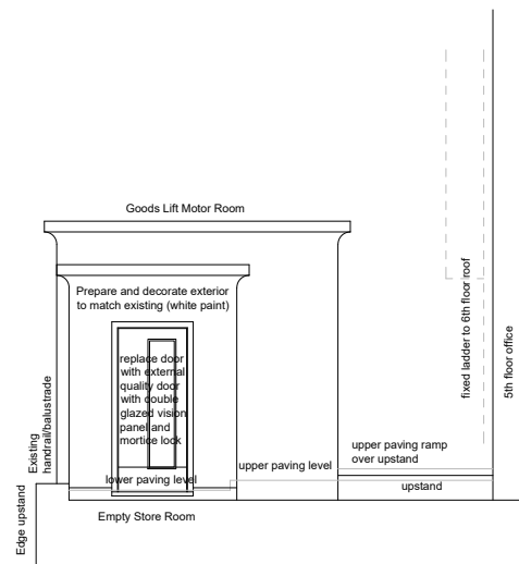
ELEVATION TO SOUTH:
