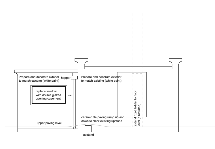
ELEVATION TO OFFICE:
