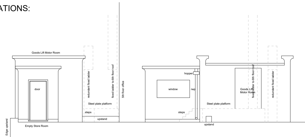
ELEVATION TO SOUTH: ELEVATION TO OFFICE:
