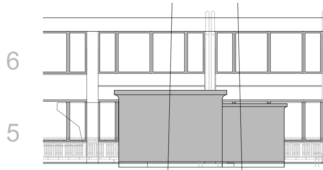
This view partially obstructed by chimney from basement: ELEVATION TO MORNINGTON CRESCENT:
