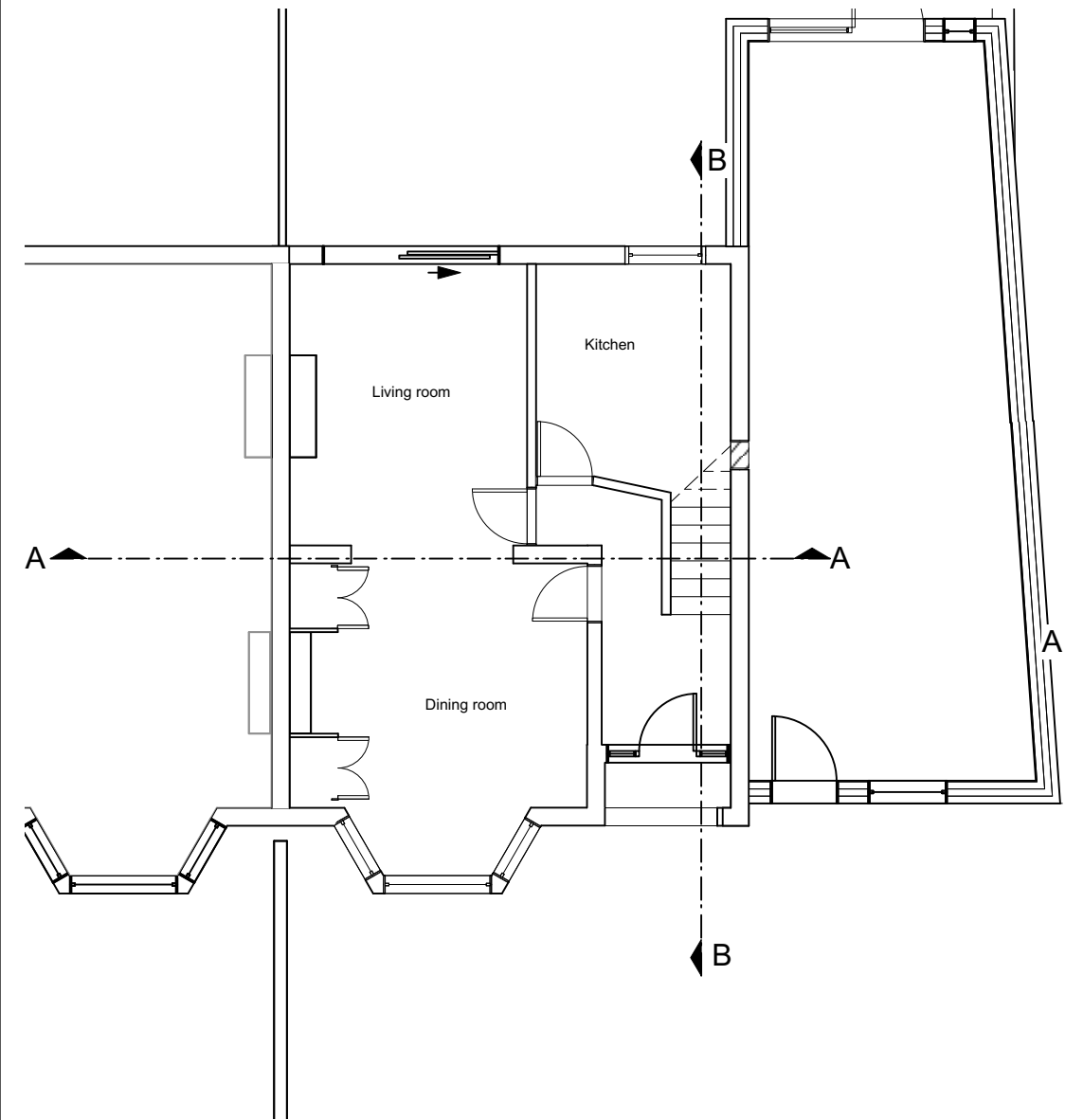
Ground floor as proposed (no change)
