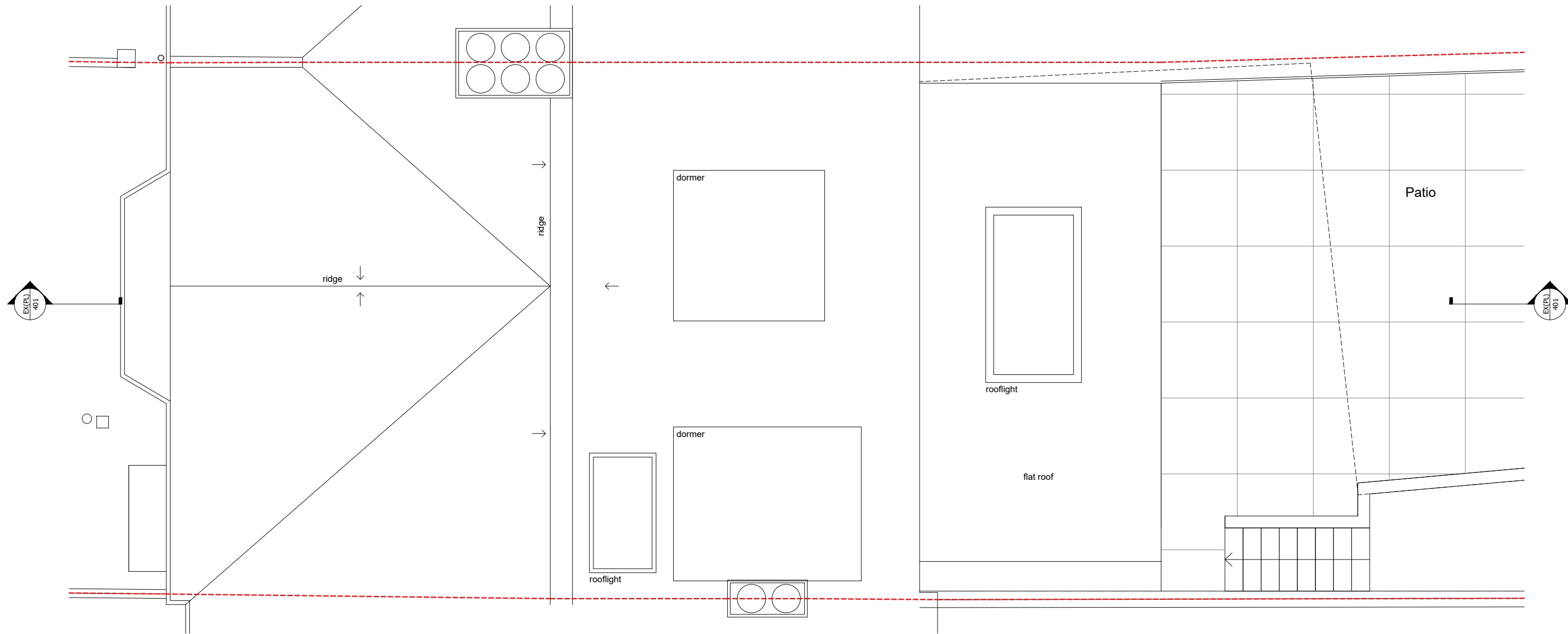
01 Proposed Roof Plan Scale 1:50 @A3
