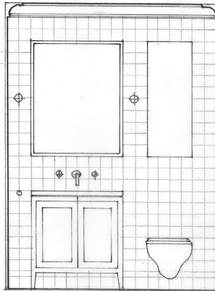
Section BB_scale: 1/20
