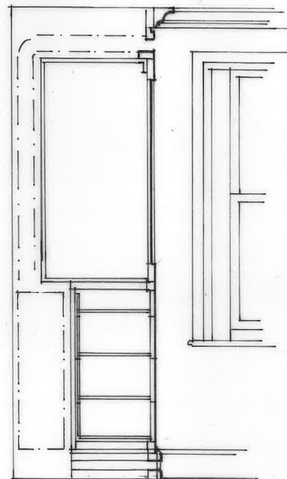
Section_scale: 1/20
