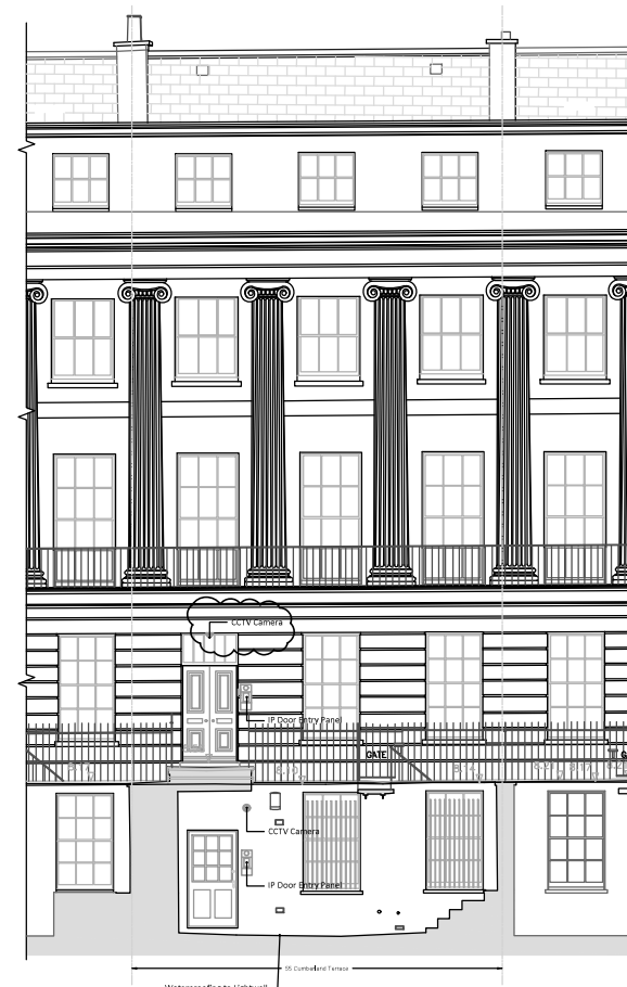
Front elevation_Proposed
