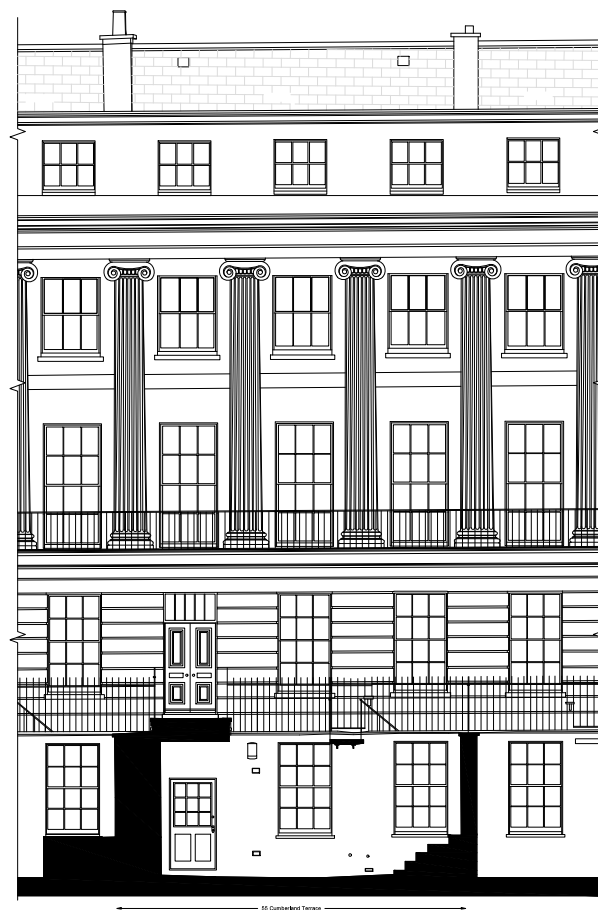
Front elevation_Existing
