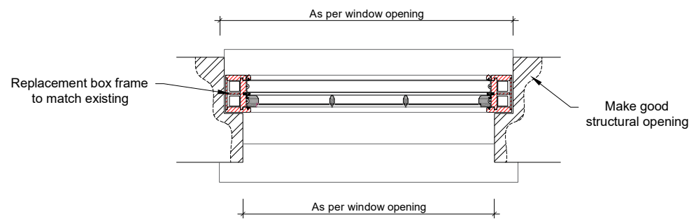
HERITAGE BOX SASH WINDOW
