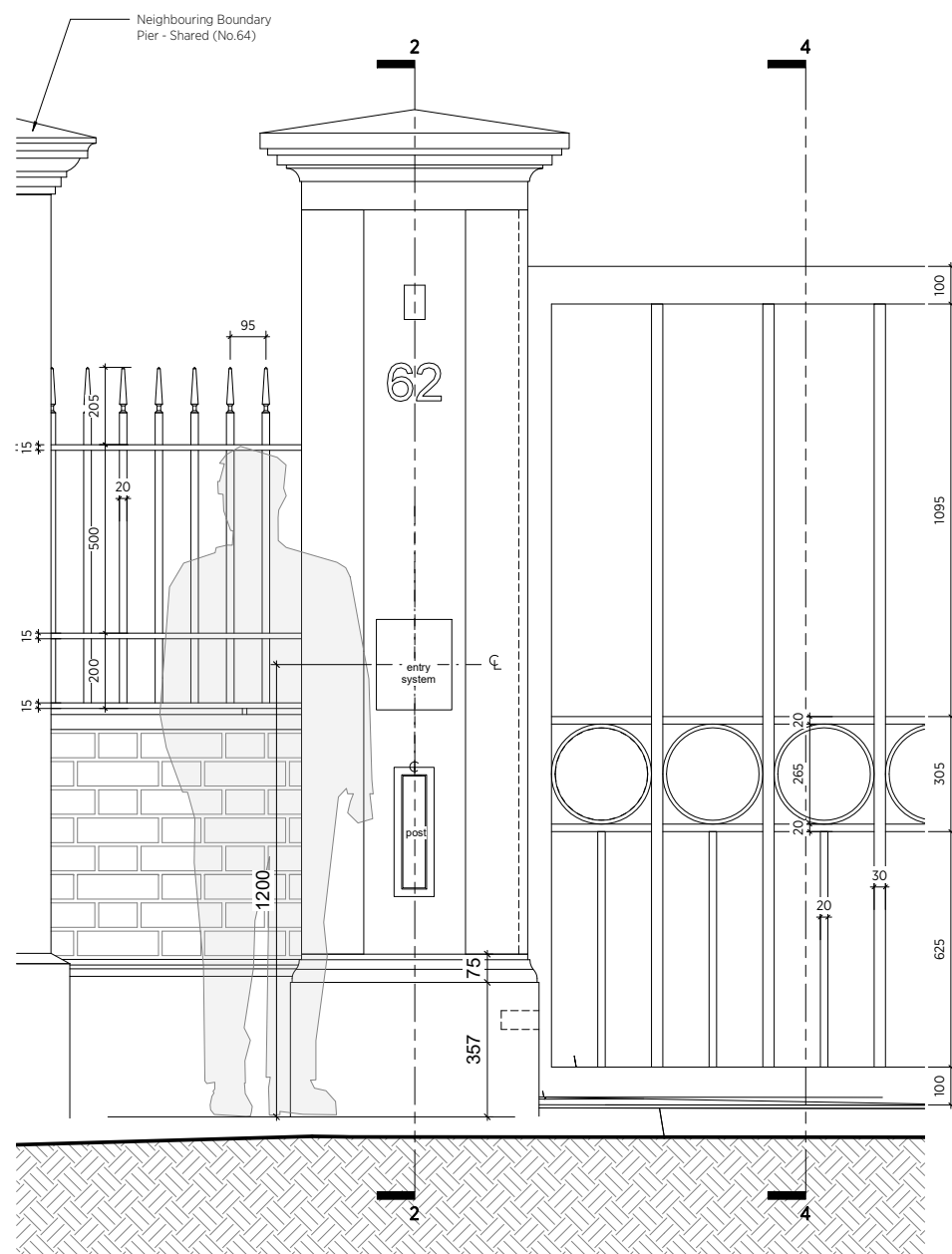
3 Gate Pier-Front Elev 1:10
