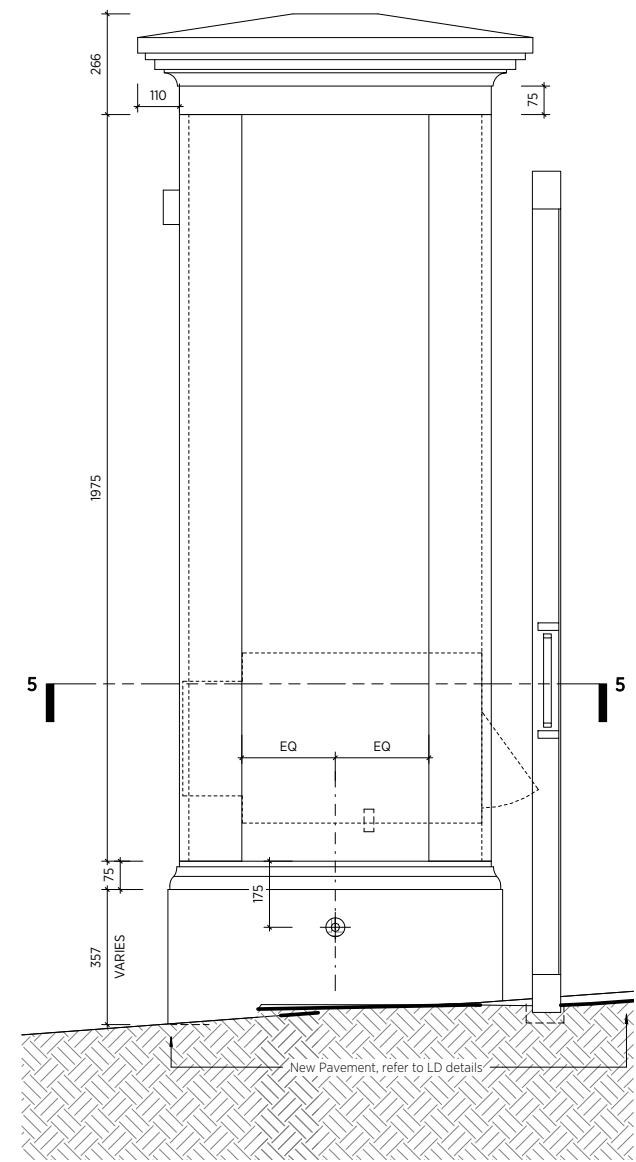
4 Gate Pier- Side Elev 1:10
