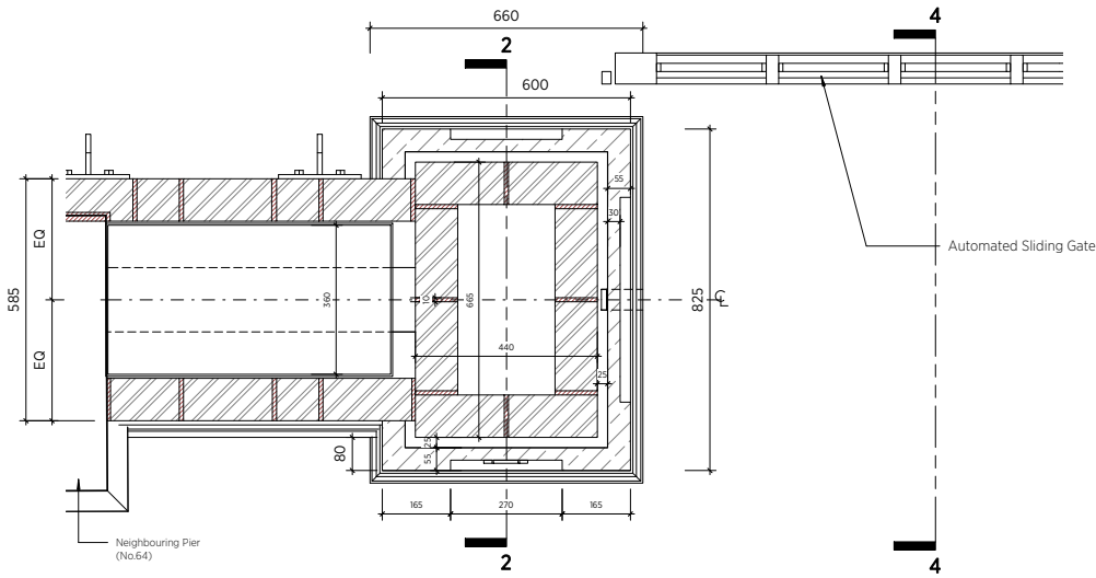
5 Gate Pier Detail-Plan 1:10
