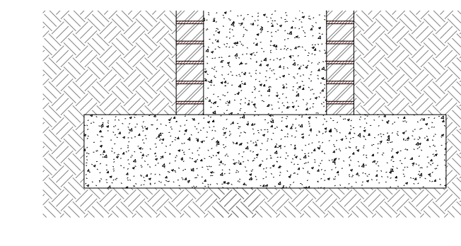
2 Gate Pier Detail Section 1:10
