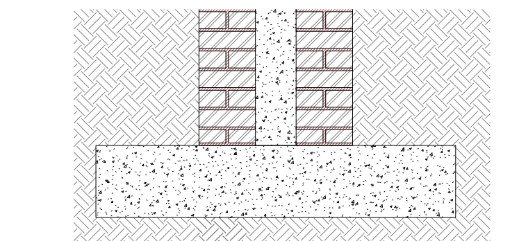
1 Boundary Wall Typical Section- Middle part between gates 1:10
