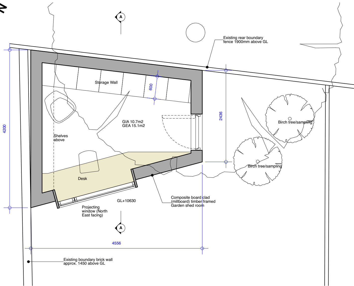
1 Proposed Garden Room Floor Plan Scale: 1:50
