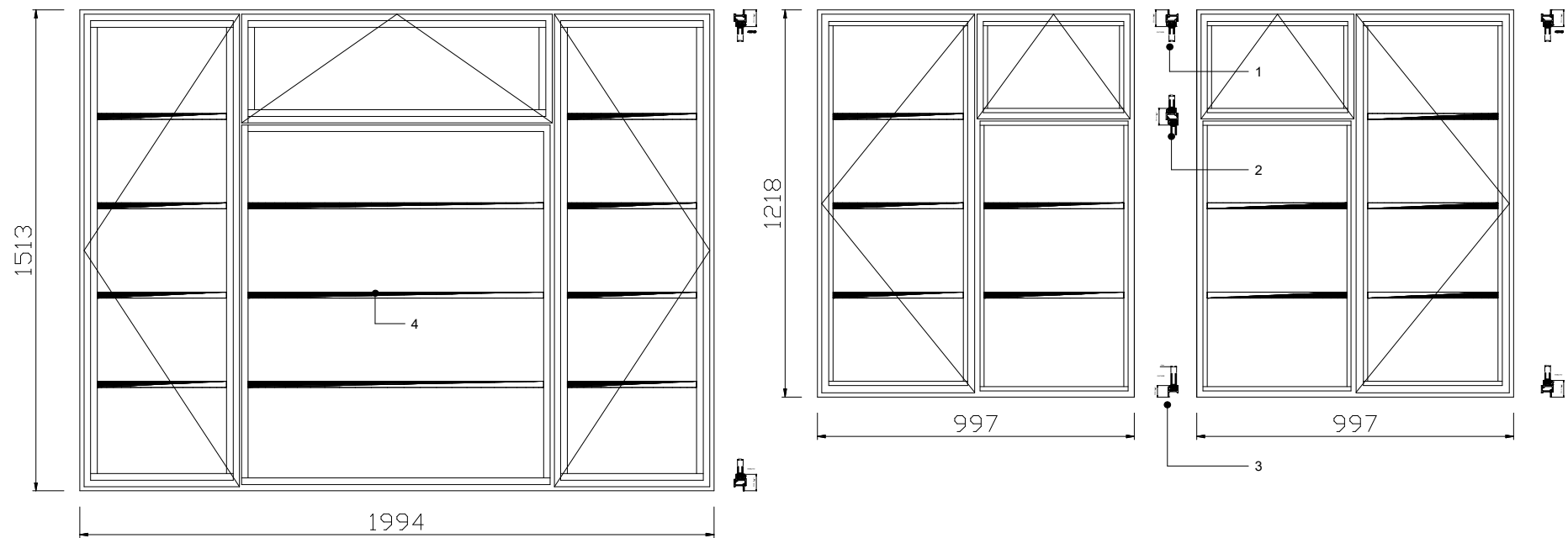
2 Proposed Crittal Windows 1 : 20
