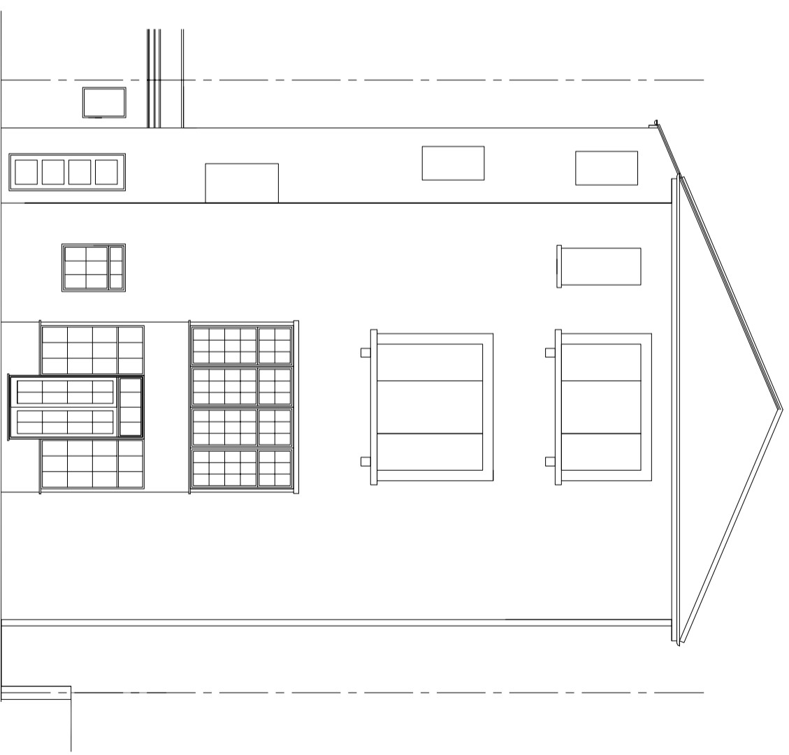
REAR ELEVATION
