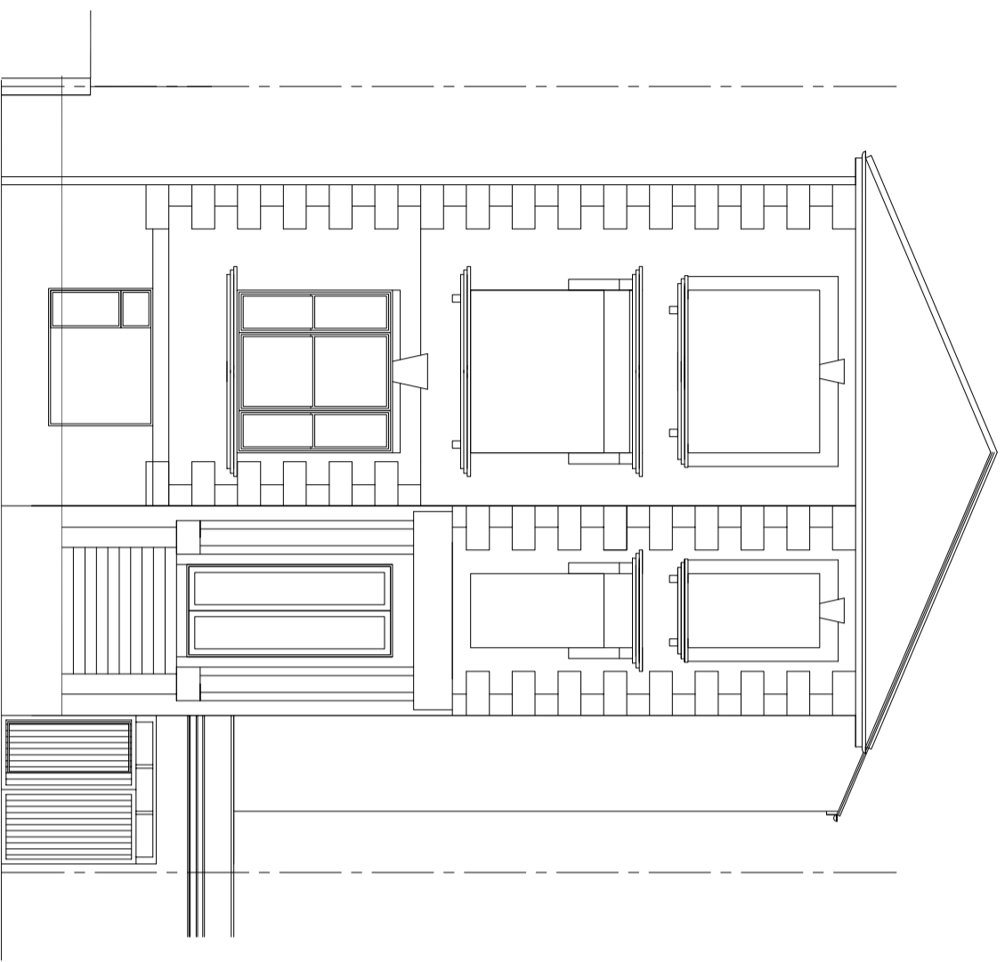
FRONT ELEVATION
