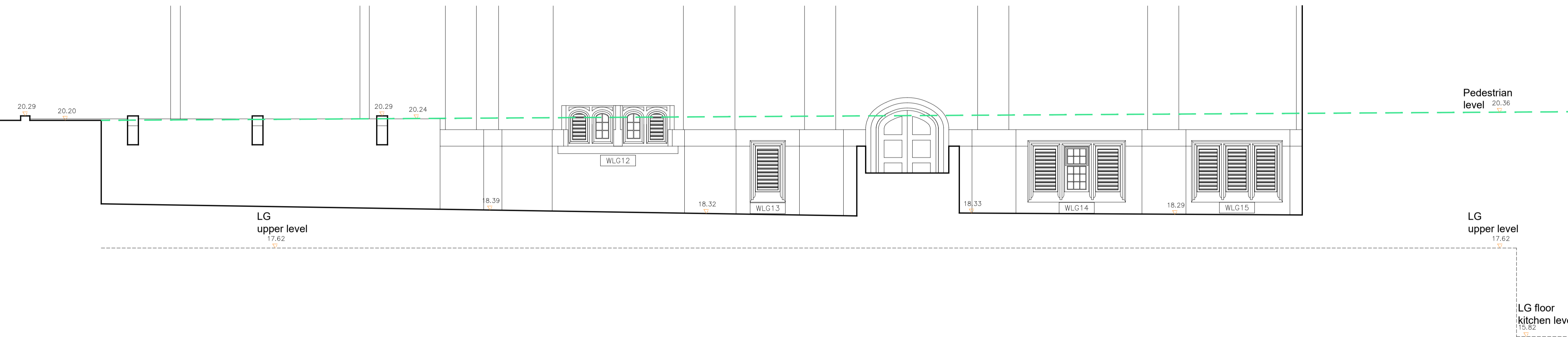
Elevation Gray's Inn Square Lightwell Windows
