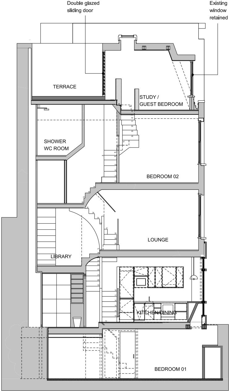
SECTION AA
