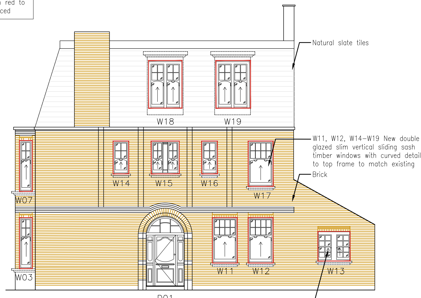
PROPOSED SIDE (MAIN) ELEVATION
