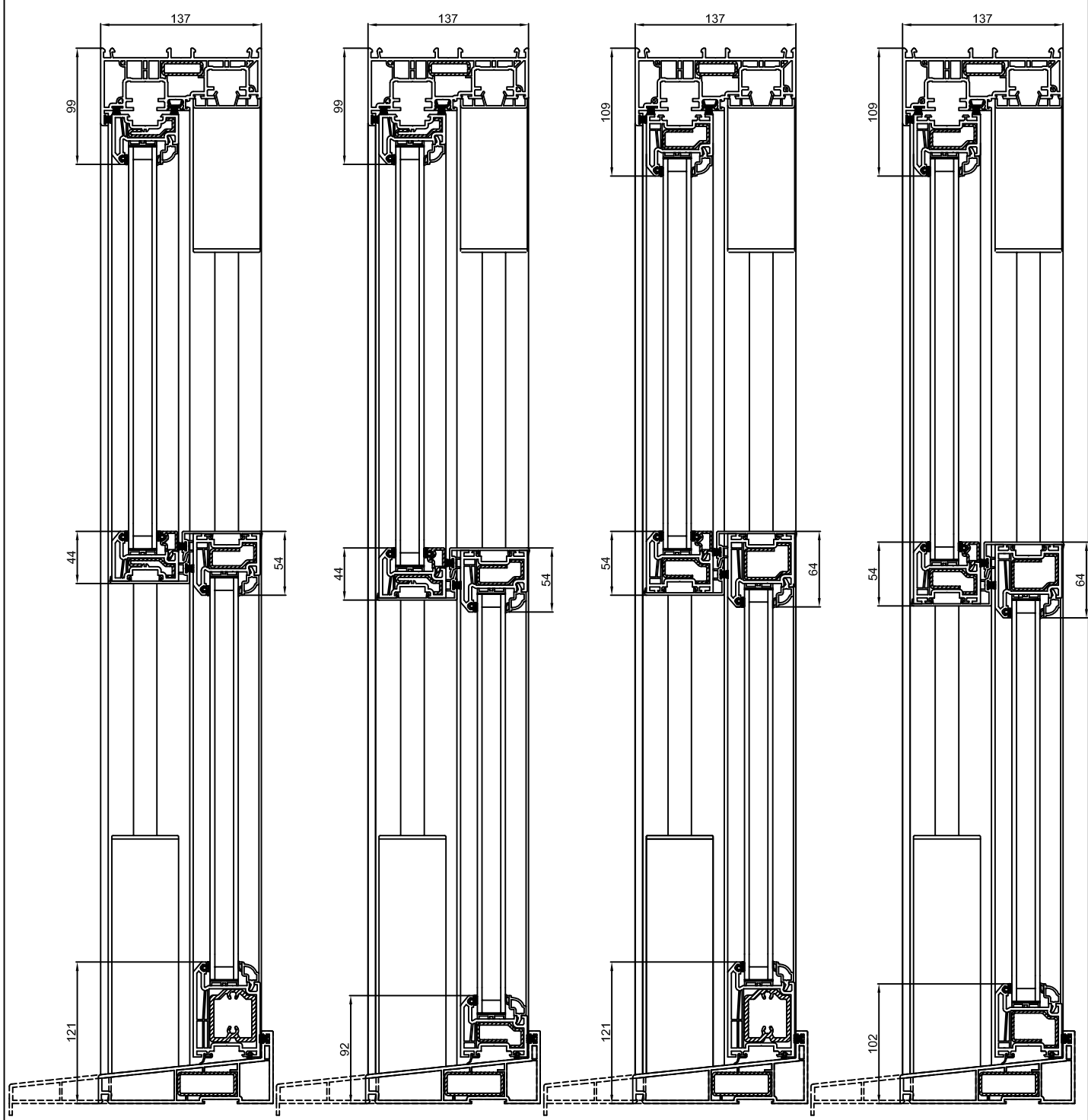
Heritage VS - Slim/Intermediate Sashes with DBR & Mech. Joint Sill
