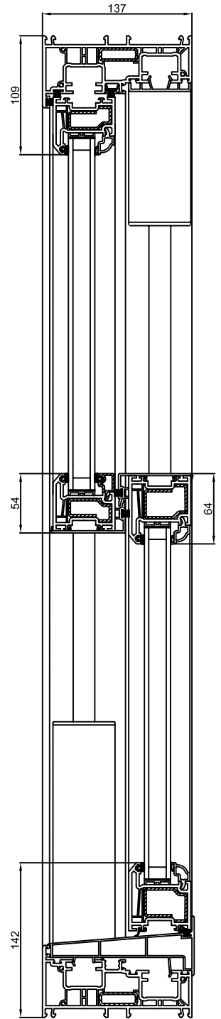
Heritage VS - Intermediate/Large Sashes with Fully Welded Frame
