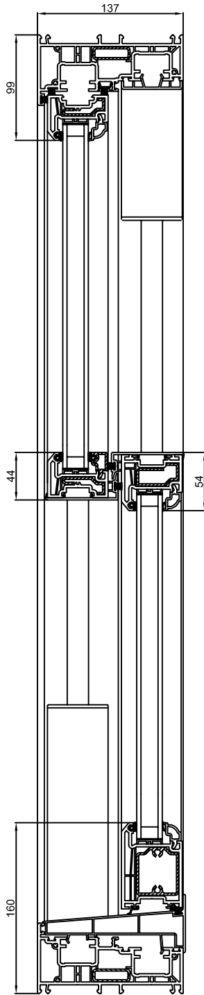
Heritage VS - Slim/Intermediate Sashes with DBR & Fully Welded Frame
