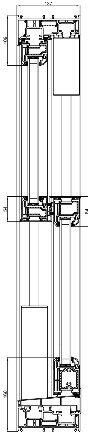
Heritage VS - Intermediate/Large Sashes with DBR & Fully Welded Frame
