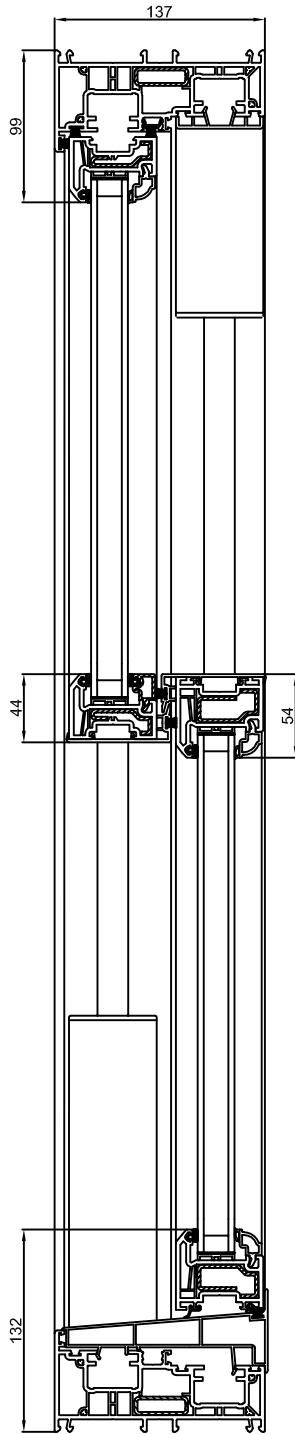
Heritage VS - Slim/Intermediate Sashes with Fully Welded Frame
