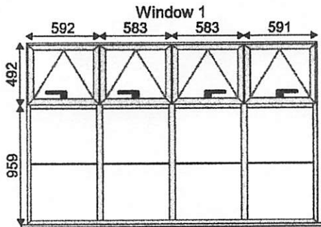
1-2349x1476 7016 Anthracite Grey - Matt 150mm Cill - KL
