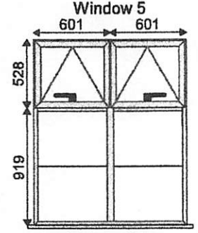
1-1202x1472 7016 Anthracite Grey - Matt 150mm Cill - KL
