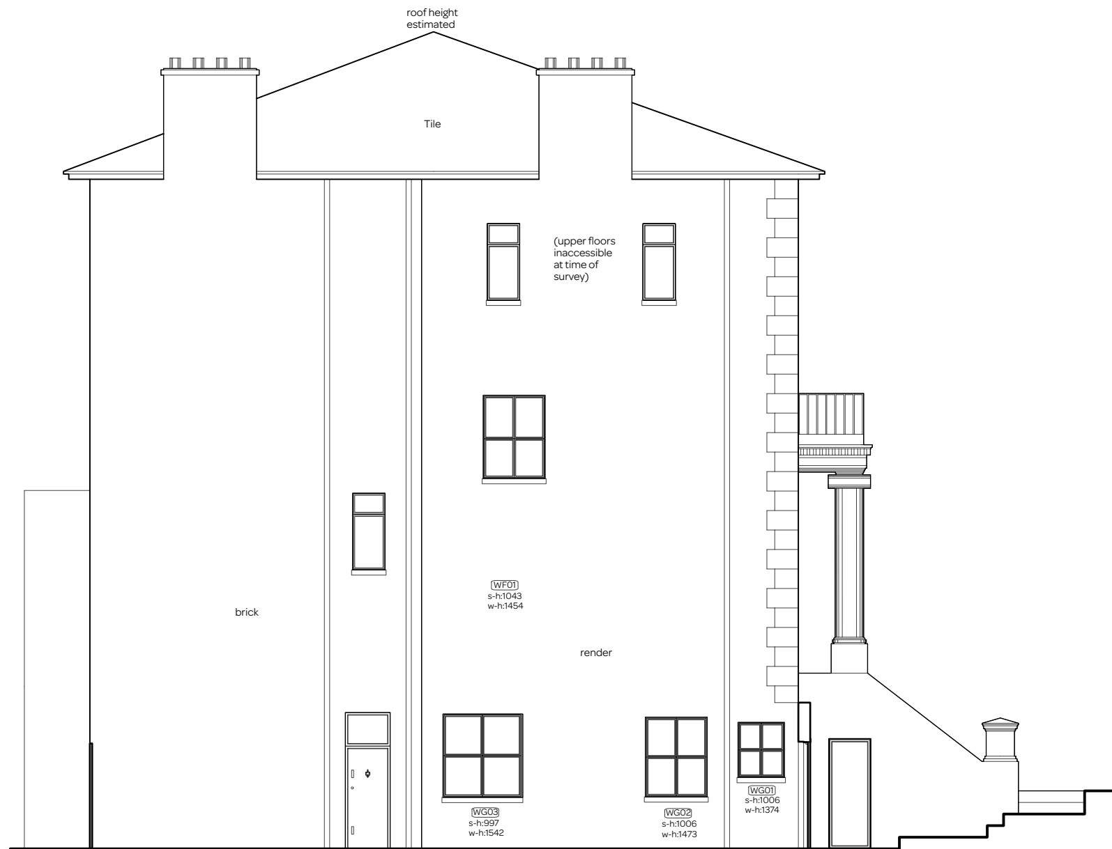
Side Elevation
