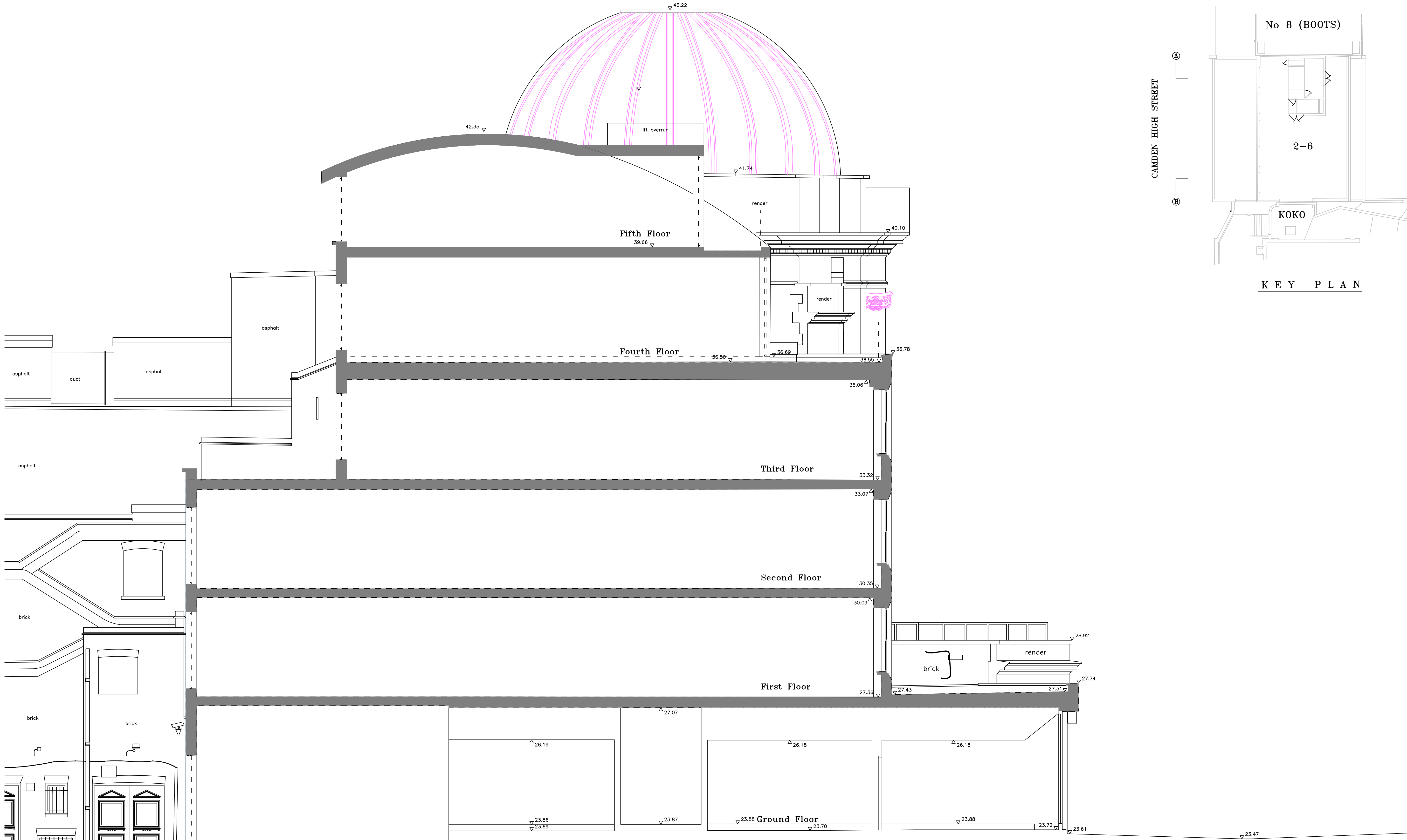
SECTION B - B 22.00m A.O.D.
