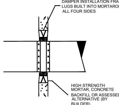
INSTALLATION OF FIRE DAMPER WITHIN BLOCK/MASONARY/CONCRETE WALL
