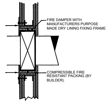
INSTALLATION OF FIRE DAMPER WITHIN DRY STUD PARTITION
