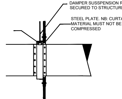
INSTALLATION OF FIRE DAMPER WITHIN CEILING VOID FIRE CURTAIN
