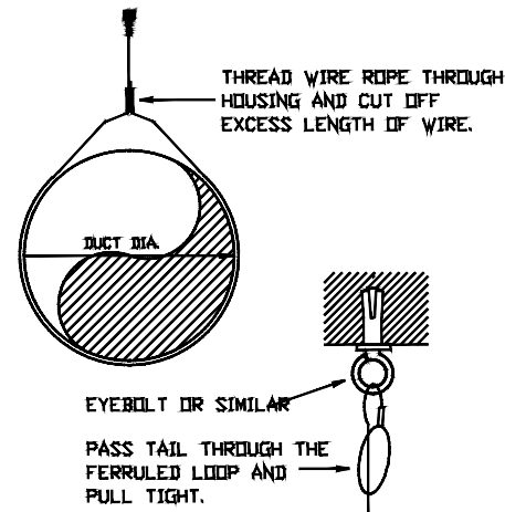
CIRCULAR SUPPORT DETAIL
