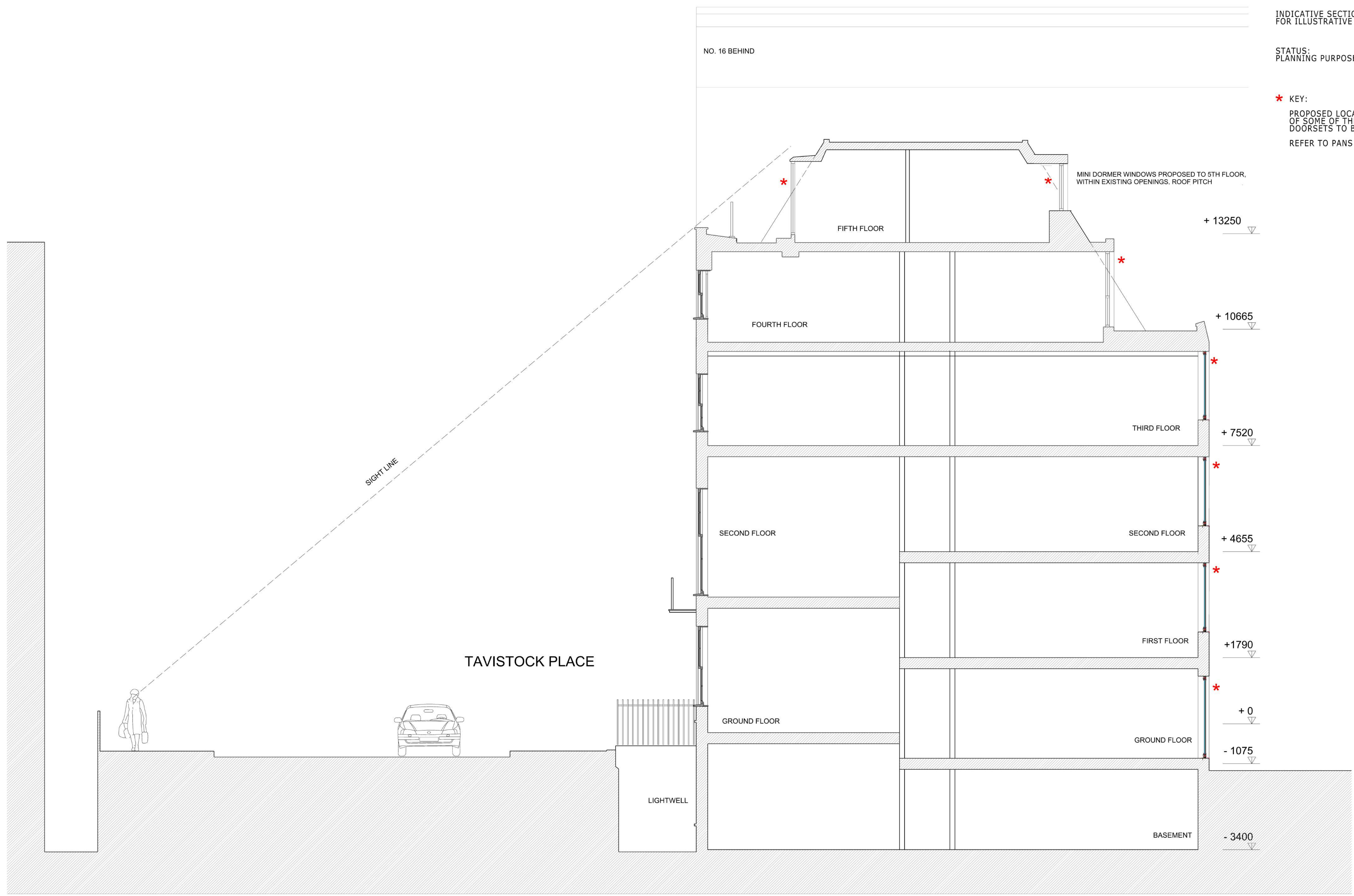
INDICATIVE SECTION
